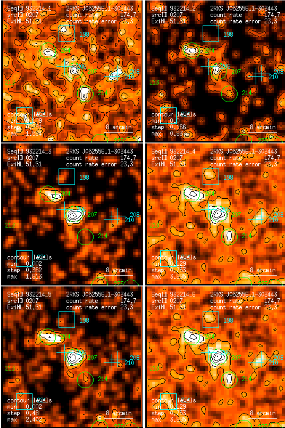
Figure 207: RASS 932214: detection 0207: band rate images, Gaussian filter: (1) PSPC channels 11 – 41, (2) 52 – 90, (3) 91 – 201, (4) 11 – 235, (5) 52 – 201, (6) 11 – 201. Broad band rates in counts/ks. Band rate contour levels in counts/ks/arcmin 2 .
