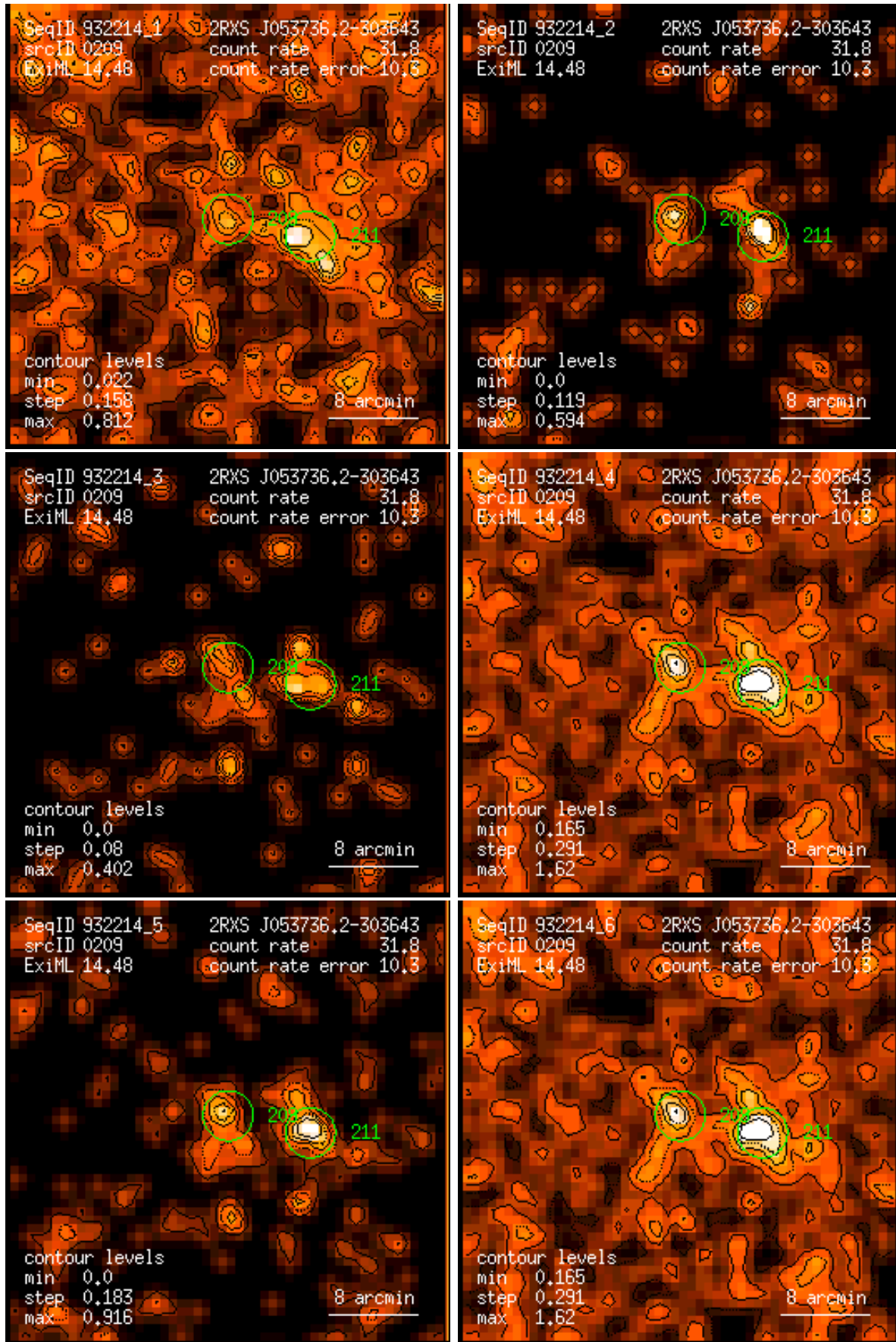
Figure 209: RASS 932214: detection 0209: band rate images, Gaussian filter: (1) PSPC channels 11 – 41, (2) 52 – 90, (3) 91 – 201, (4) 11 – 235, (5) 52 – 201, (6) 11 – 201. Broad band rates in counts/ks. Band rate contour levels in counts/ks/arcmin 2 .
