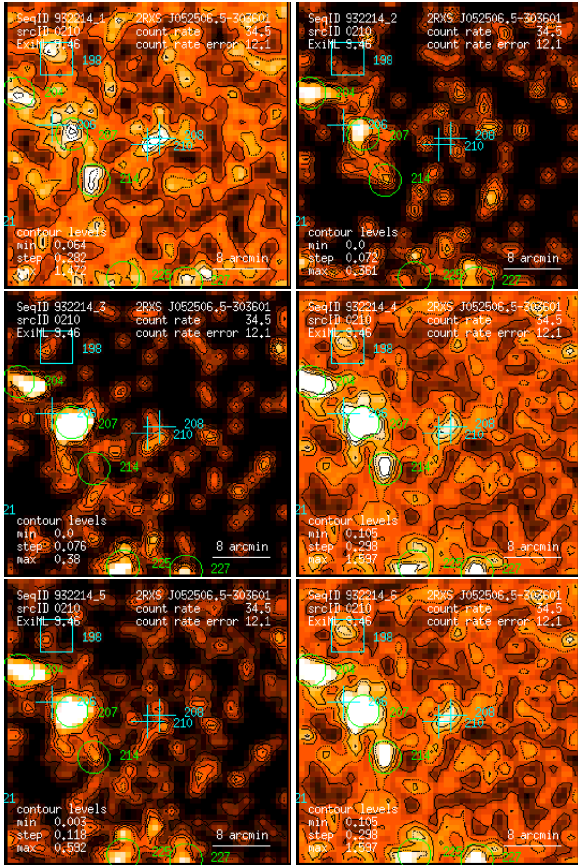
Figure 210: RASS 932214: detection 0210: band rate images, Gaussian filter: (1) PSPC channels 11 – 41, (2) 52 – 90, (3) 91 – 201, (4) 11 – 235, (5) 52 – 201, (6) 11 – 201. Broad band rates in counts/ks. Band rate contour levels in counts/ks/arcmin 2 .
