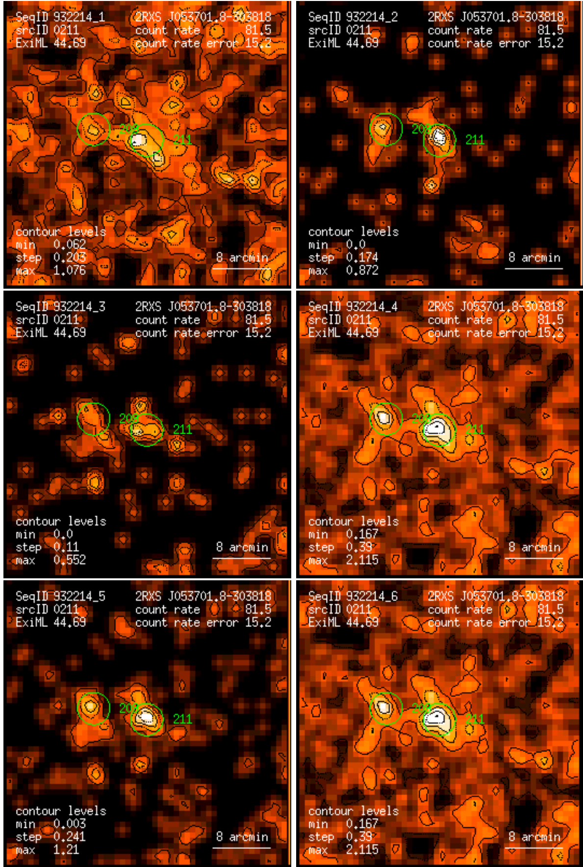
Figure 211: RASS 932214: detection 0211: band rate images, Gaussian filter: (1) PSPC channels 11 – 41, (2) 52 – 90, (3) 91 – 201, (4) 11 – 235, (5) 52 – 201, (6) 11 – 201. Broad band rates in counts/ks. Band rate contour levels in counts/ks/arcmin 2 .
