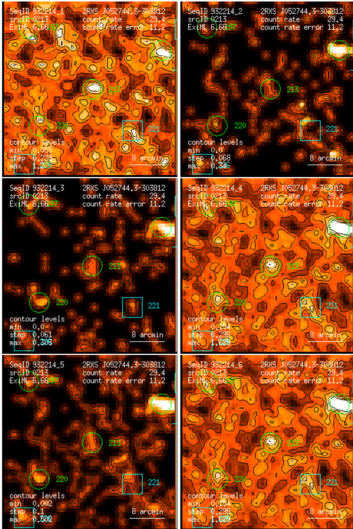
Figure 213: RASS 932214: detection 0213: band rate images, Gaussian filter: (1) PSPC channels 11 – 41, (2) 52 – 90, (3) 91 – 201, (4) 11 – 235, (5) 52 – 201, (6) 11 – 201. Broad band rates in counts/ks. Band rate contour levels in counts/ks/arcmin 2 .
