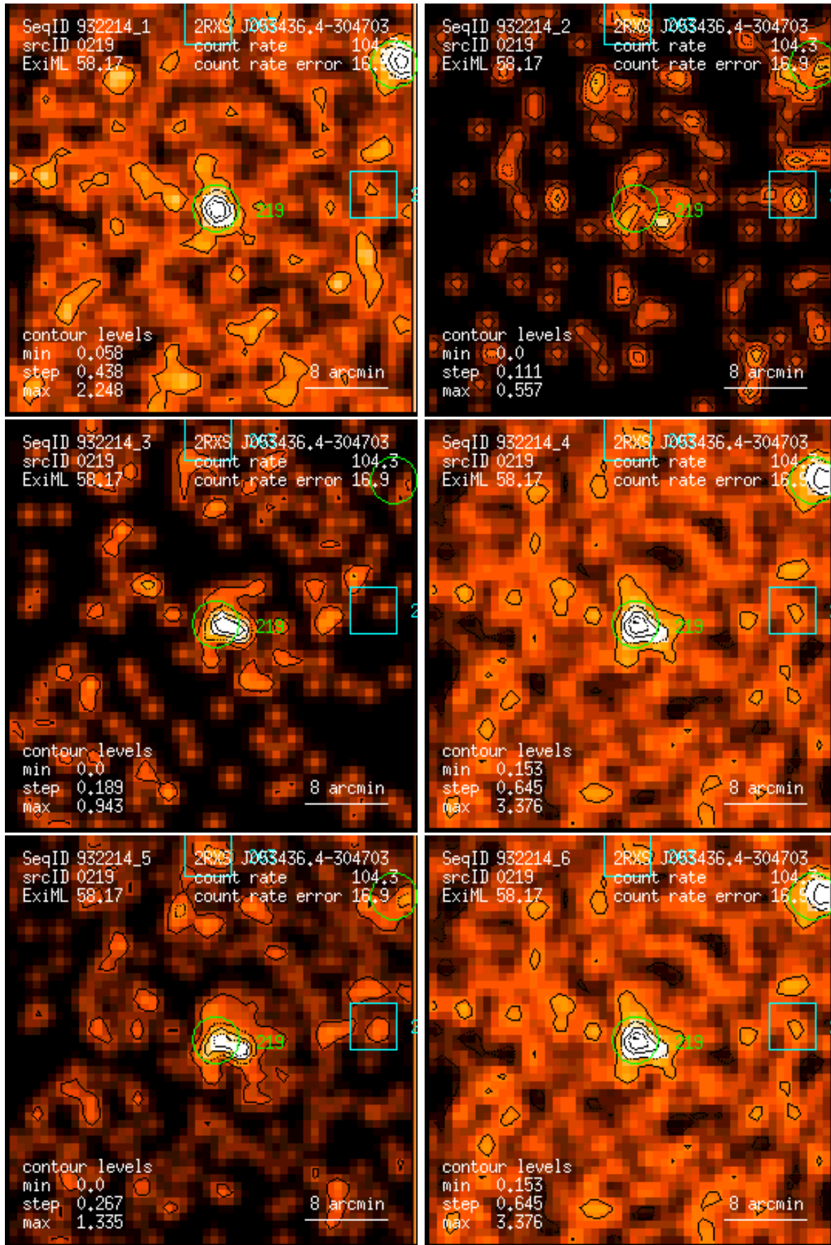
Figure 219: RASS 932214: detection 0219: band rate images, Gaussian filter: (1) PSPC channels 11 – 41, (2) 52 – 90, (3) 91 – 201, (4) 11 – 235, (5) 52 – 201, (6) 11 – 201. Broad band rates in counts/ks. Band rate contour levels in counts/ks/arcmin 2 .
