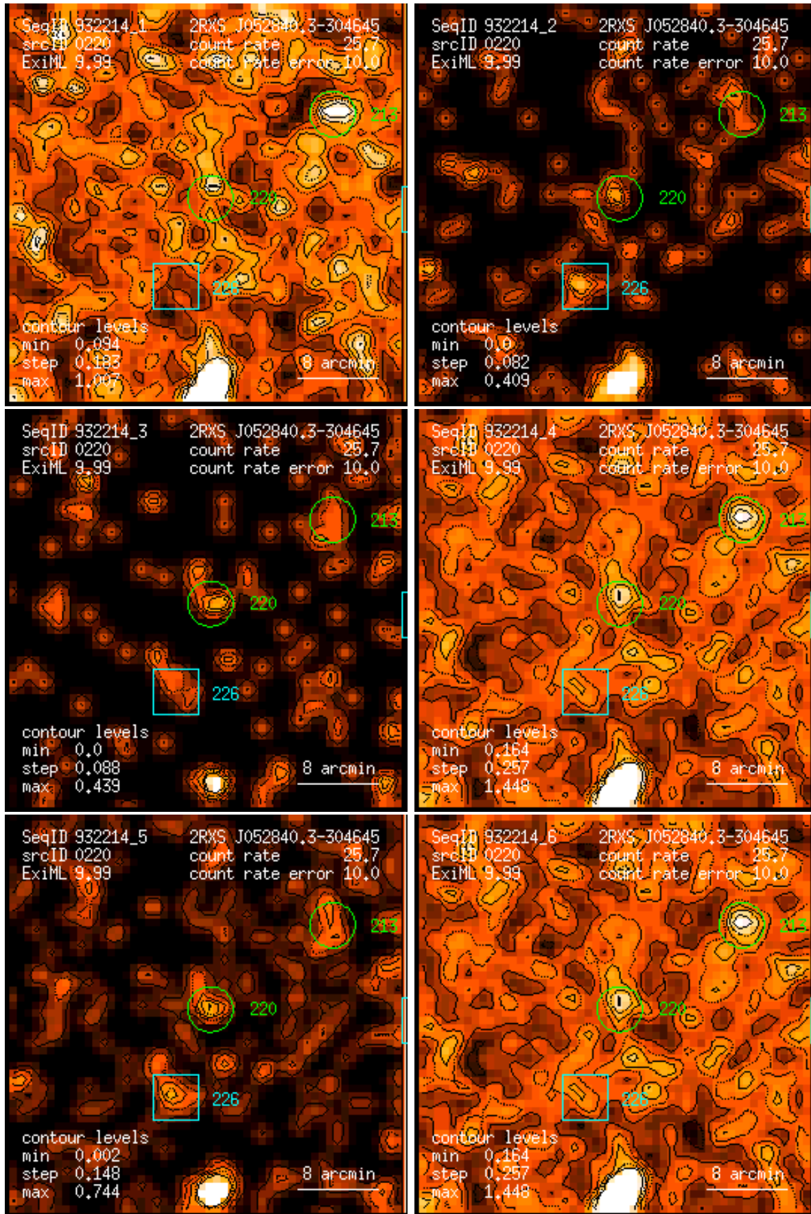
Figure 220: RASS 932214: detection 0220: band rate images, Gaussian filter: (1) PSPC channels 11 – 41, (2) 52 – 90, (3) 91 – 201, (4) 11 – 235, (5) 52 – 201, (6) 11 – 201. Broad band rates in counts/ks. Band rate contour levels in counts/ks/arcmin 2 .
