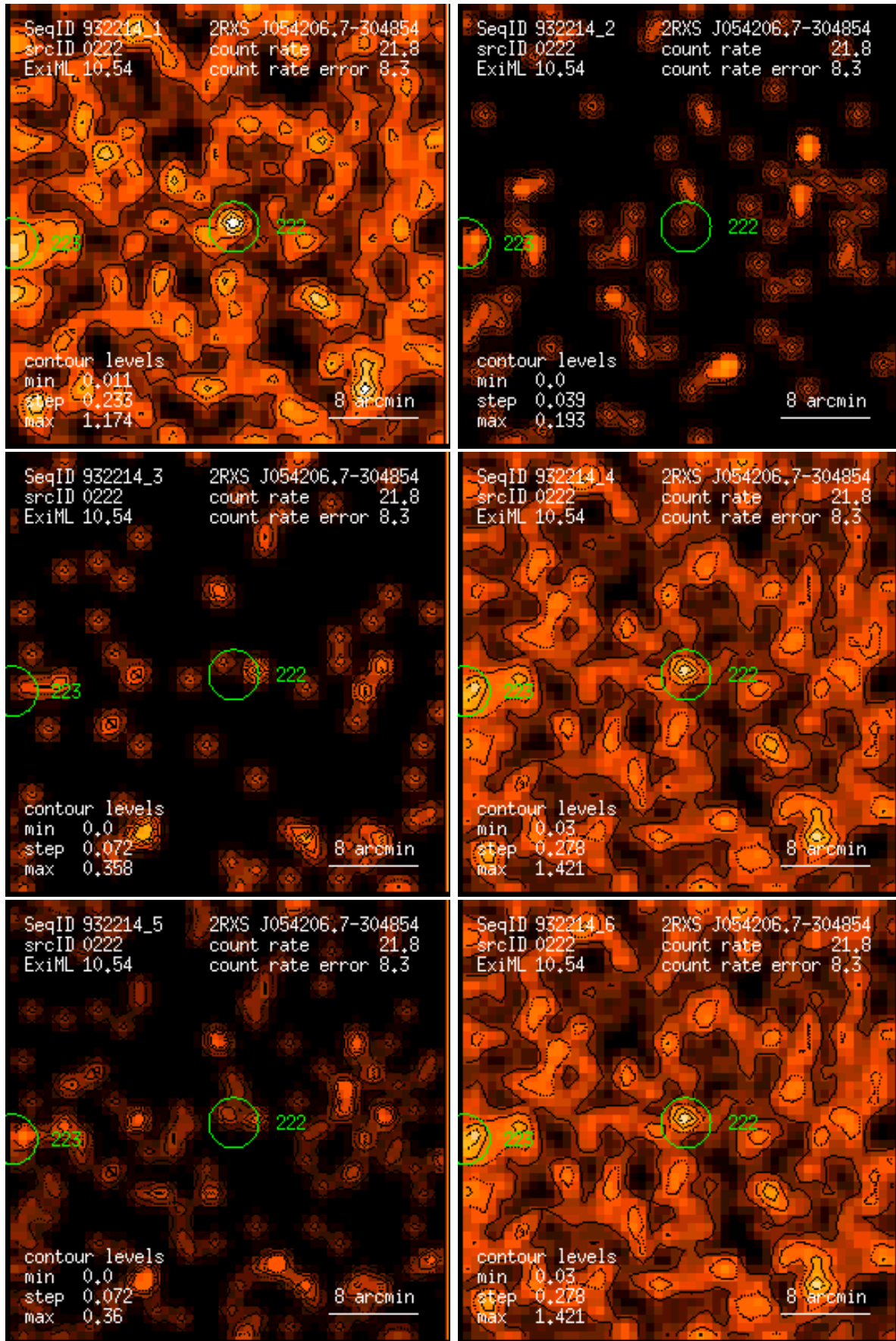
Figure 222: RASS 932214: detection 0222: band rate images, Gaussian filter: (1) PSPC channels 11 – 41, (2) 52 – 90, (3) 91 – 201, (4) 11 – 235, (5) 52 – 201, (6) 11 – 201. Broad band rates in counts/ks. Band rate contour levels in counts/ks/arcmin 2 .
