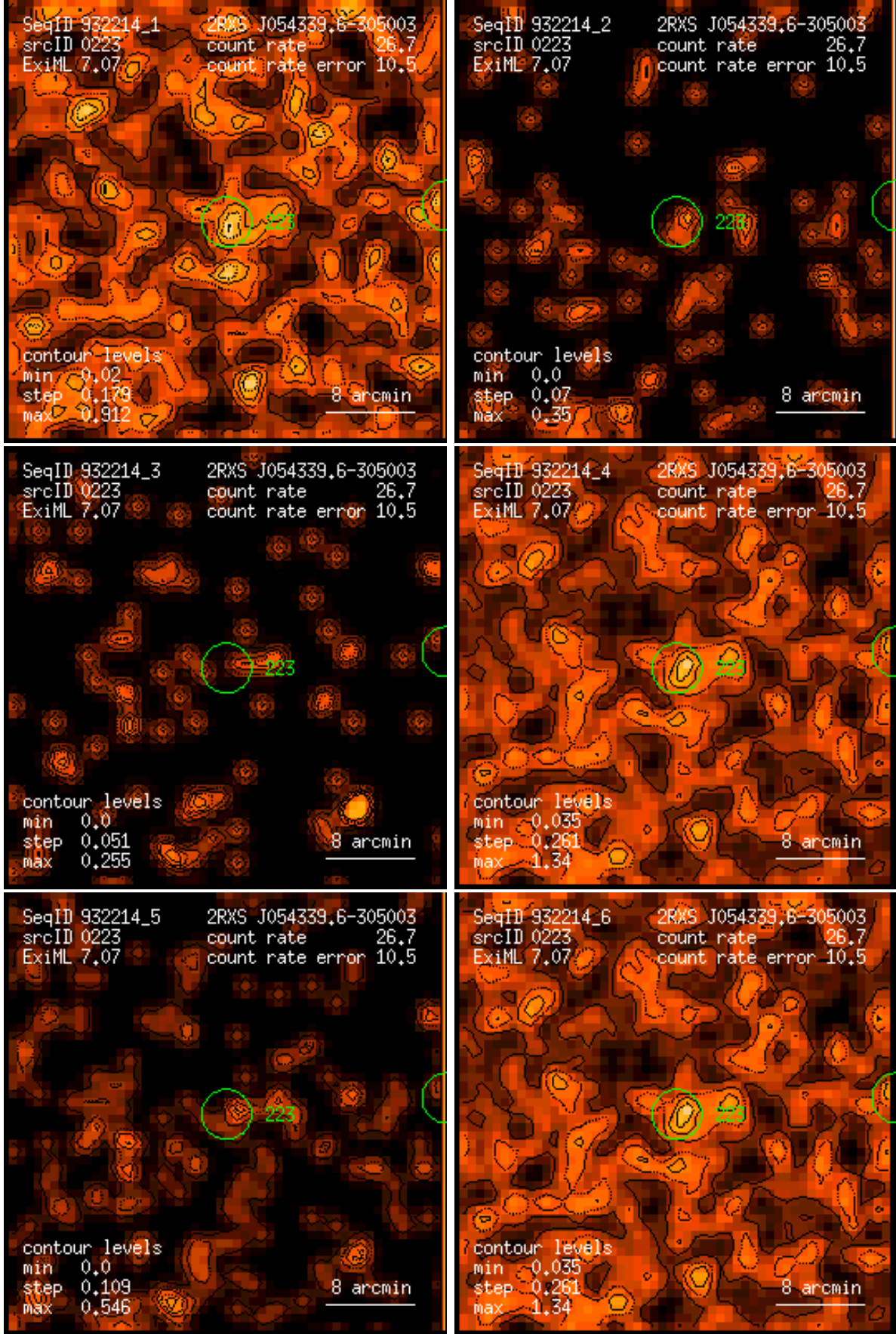
Figure 223: RASS 932214: detection 0223: band rate images, Gaussian filter: (1) PSPC channels 11 – 41, (2) 52 – 90, (3) 91 – 201, (4) 11 – 235, (5) 52 – 201, (6) 11 – 201. Broad band rates in counts/ks. Band rate contour levels in counts/ks/arcmin 2 .
