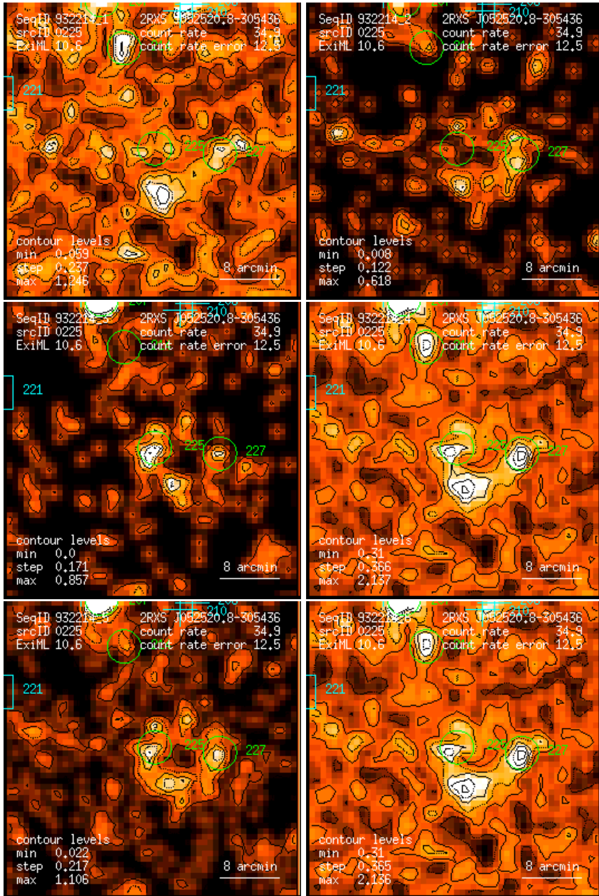
Figure 225: RASS 932214: detection 0225: band rate images, Gaussian filter: (1) PSPC channels 11 – 41, (2) 52 – 90, (3) 91 – 201, (4) 11 – 235, (5) 52 – 201, (6) 11 – 201. Broad band rates in counts/ks. Band rate contour levels in counts/ks/arcmin 2 .
