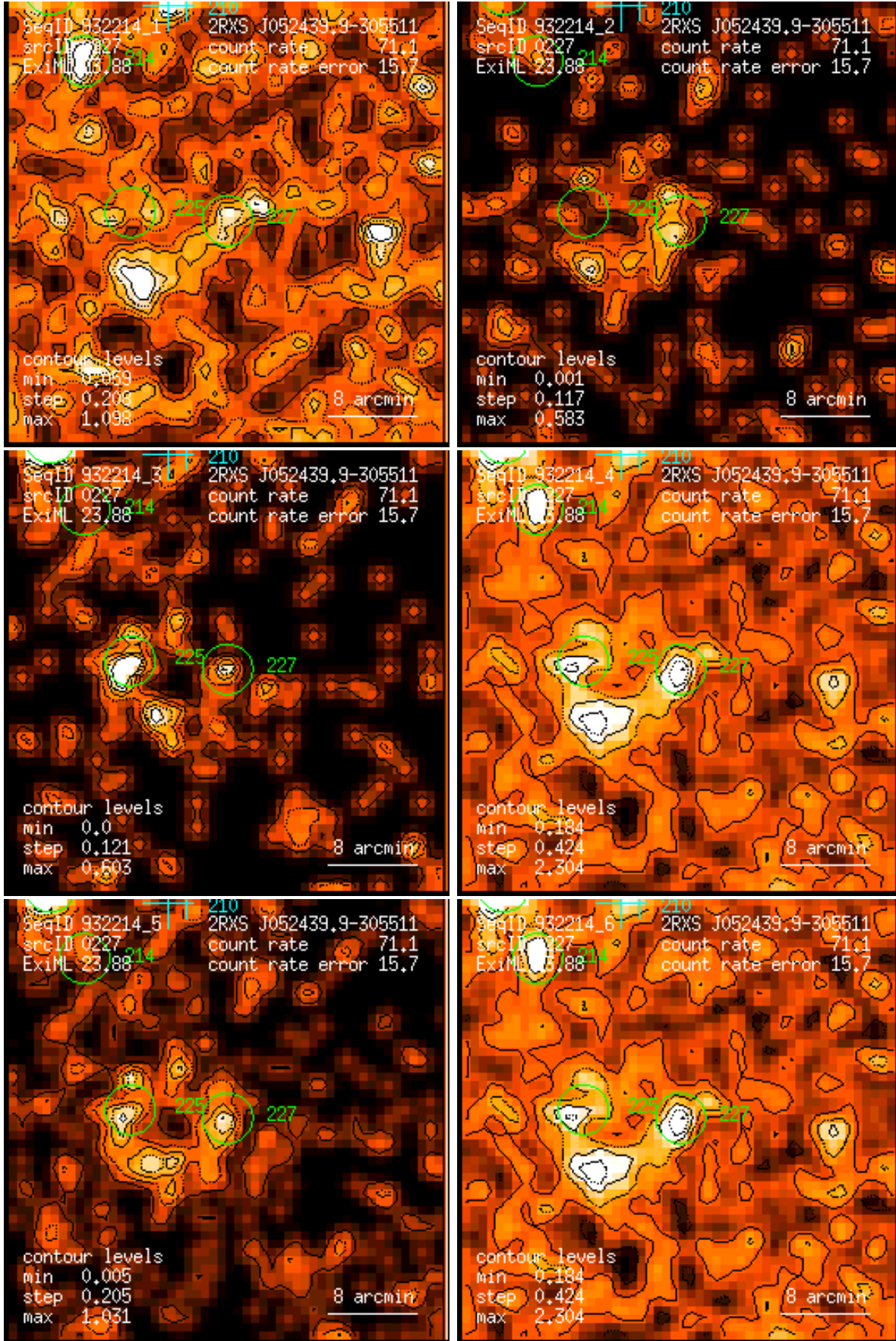
Figure 227: RASS 932214: detection 0227: band rate images, Gaussian filter: (1) PSPC channels 11 – 41, (2) 52 – 90, (3) 91 – 201, (4) 11 – 235, (5) 52 – 201, (6) 11 – 201. Broad band rates in counts/ks. Band rate contour levels in counts/ks/arcmin 2 .
