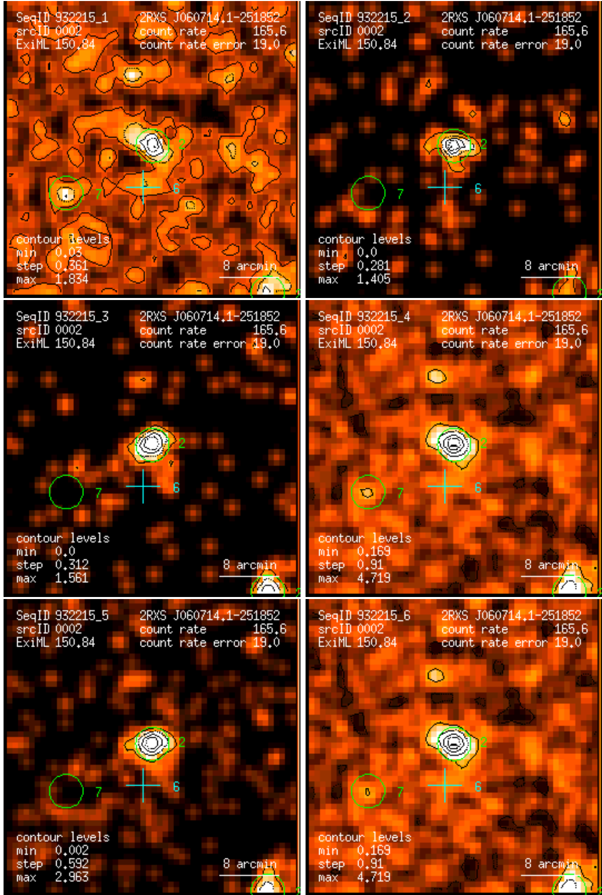
Figure 2: RASS 932215: detection 0002: band rate images, Gaussian filter: (1) PSPC channels 11 – 41, (2) 52 – 90, (3) 91 – 201, (4) 11 – 235, (5) 52 – 201, (6) 11 – 201. Broad band rates in counts/ks. Band rate contour levels in counts/ks/arcmin 2 .
