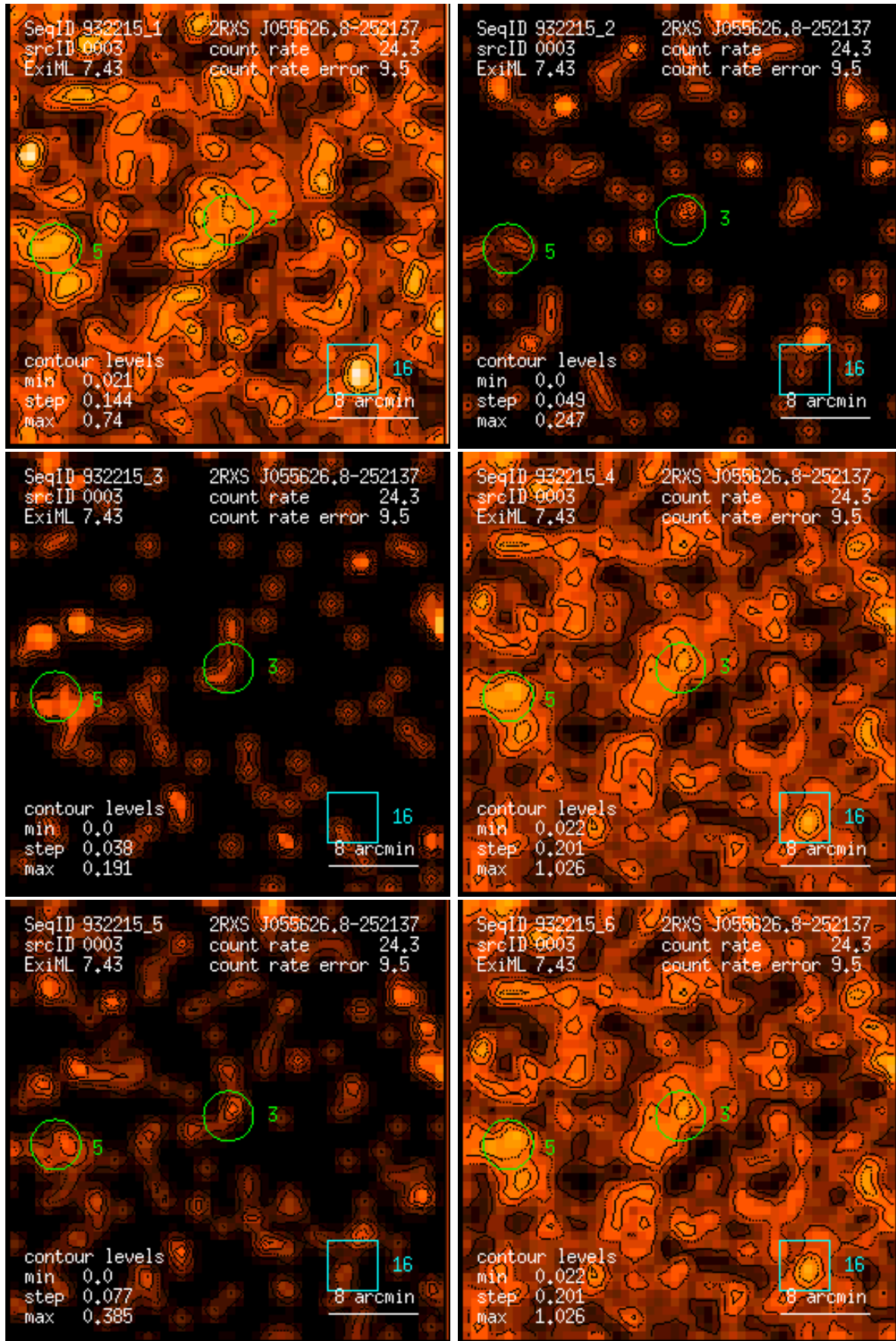
Figure 3: RASS 932215: detection 0003: band rate images, Gaussian filter: (1) PSPC channels 11 – 41, (2) 52 – 90, (3) 91 – 201, (4) 11 – 235, (5) 52 – 201, (6) 11 – 201. Broad band rates in counts/ks. Band rate contour levels in counts/ks/arcmin 2 .
