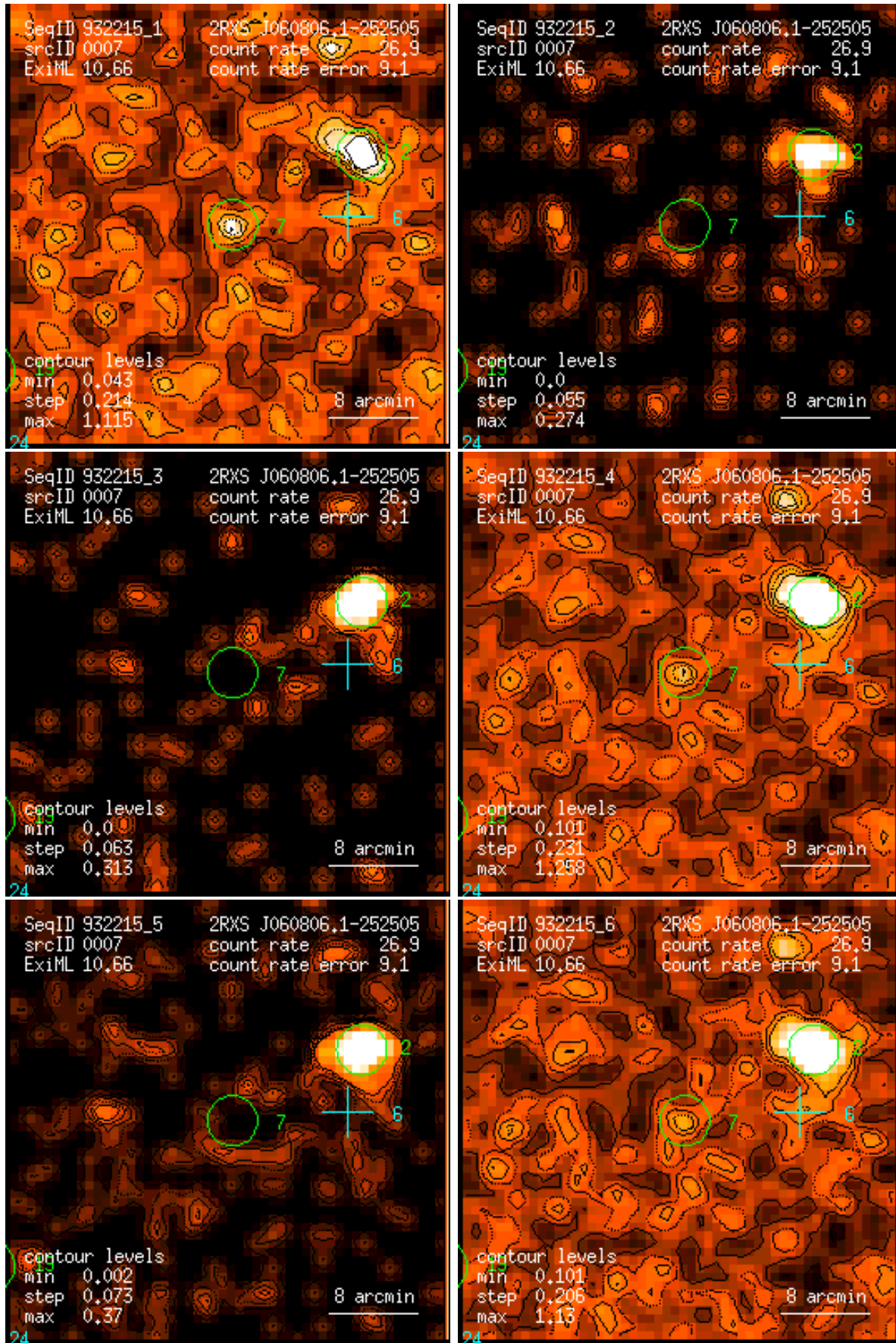
Figure 7: RASS 932215: detection 0007: band rate images, Gaussian filter: (1) PSPC channels 11 – 41, (2) 52 – 90, (3) 91 – 201, (4) 11 – 235, (5) 52 – 201, (6) 11 – 201. Broad band rates in counts/ks. Band rate contour levels in counts/ks/arcmin 2 .
