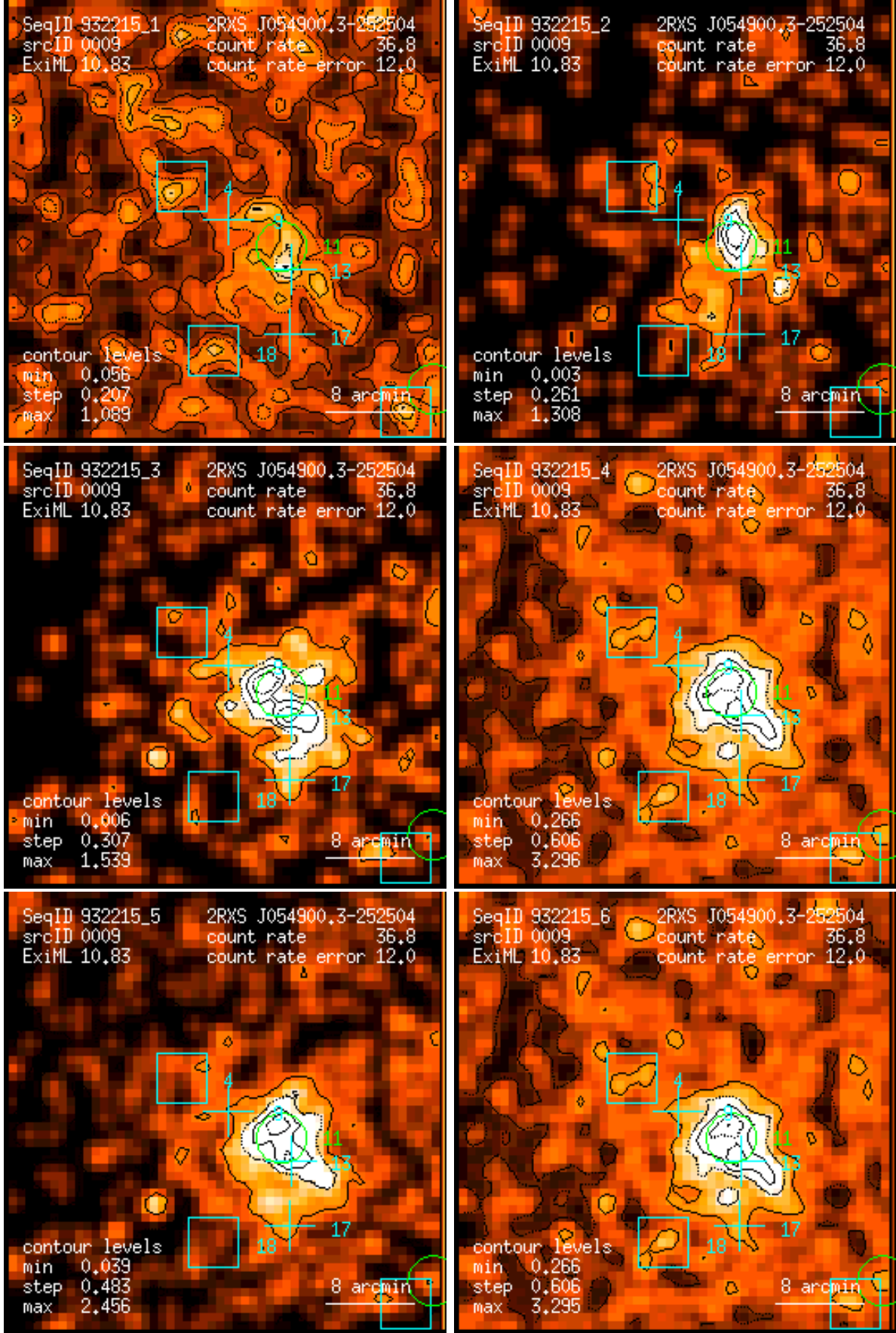
Figure 9: RASS 932215: detection 0009: band rate images, Gaussian filter: (1) PSPC channels 11 – 41, (2) 52 – 90, (3) 91 – 201, (4) 11 – 235, (5) 52 – 201, (6) 11 – 201. Broad band rates in counts/ks. Band rate contour levels in counts/ks/arcmin 2 .
