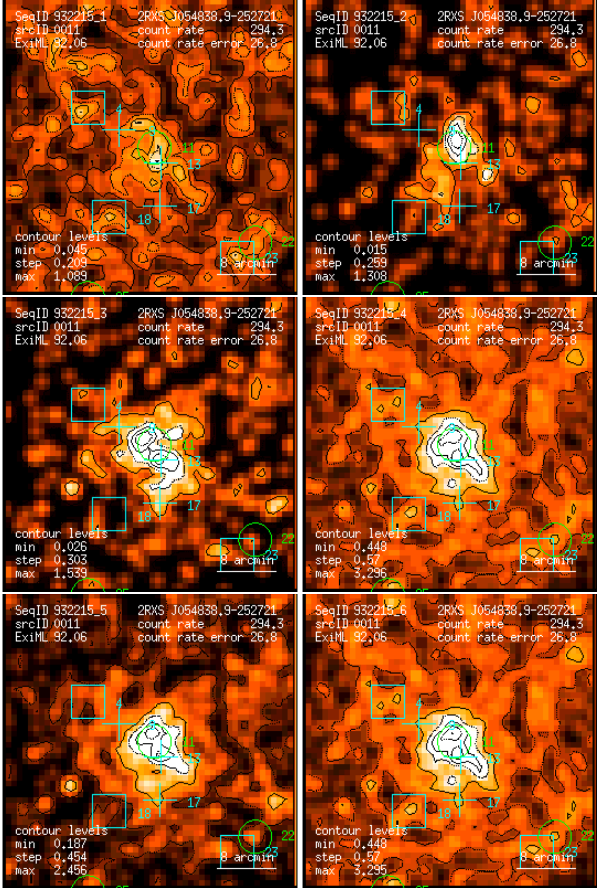
Figure 11: RASS 932215: detection 0011: band rate images, Gaussian filter: (1) PSPC channels 11 – 41, (2) 52 – 90, (3) 91 – 201, (4) 11 – 235, (5) 52 – 201, (6) 11 – 201. Broad band rates in counts/ks. Band rate contour levels in counts/ks/arcmin 2 .
