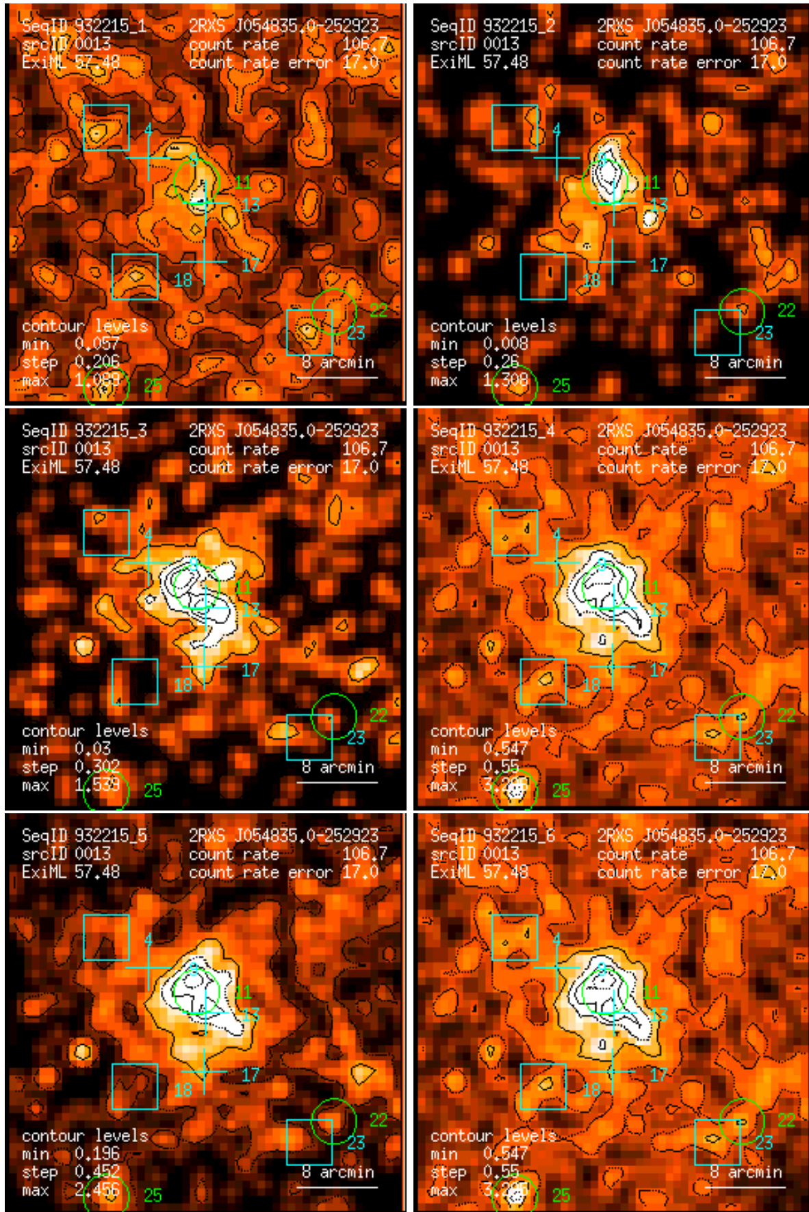
Figure 13: RASS 932215: detection 0013: band rate images, Gaussian filter: (1) PSPC channels 11 – 41, (2) 52 – 90, (3) 91 – 201, (4) 11 – 235, (5) 52 – 201, (6) 11 – 201. Broad band rates in counts/ks. Band rate contour levels in counts/ks/arcmin 2 .
