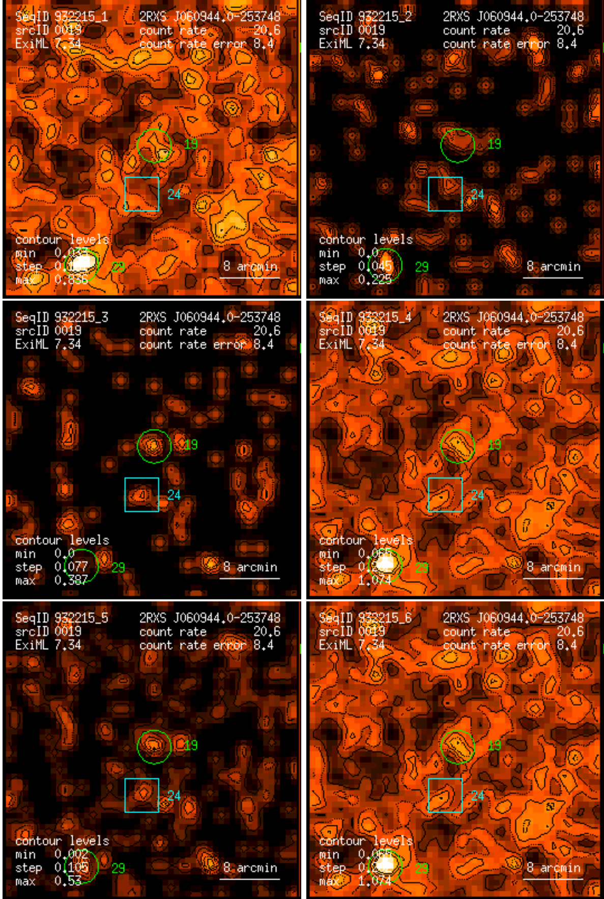
Figure 19: RASS 932215: detection 0019: band rate images, Gaussian filter: (1) PSPC channels 11 – 41, (2) 52 – 90, (3) 91 – 201, (4) 11 – 235, (5) 52 – 201, (6) 11 – 201. Broad band rates in counts/ks. Band rate contour levels in counts/ks/arcmin 2 .
