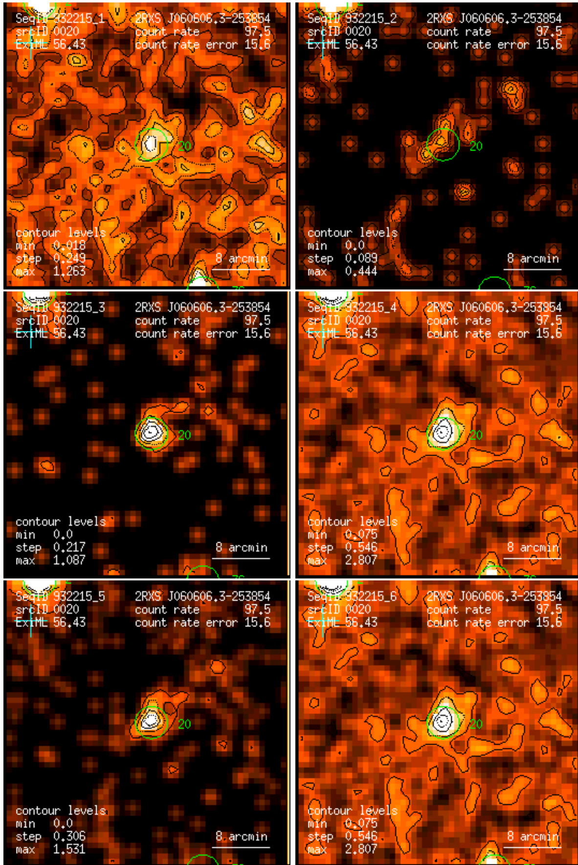
Figure 20: RASS 932215: detection 0020: band rate images, Gaussian filter: (1) PSPC channels 11 – 41, (2) 52 – 90, (3) 91 – 201, (4) 11 – 235, (5) 52 – 201, (6) 11 – 201. Broad band rates in counts/ks. Band rate contour levels in counts/ks/arcmin 2 .
