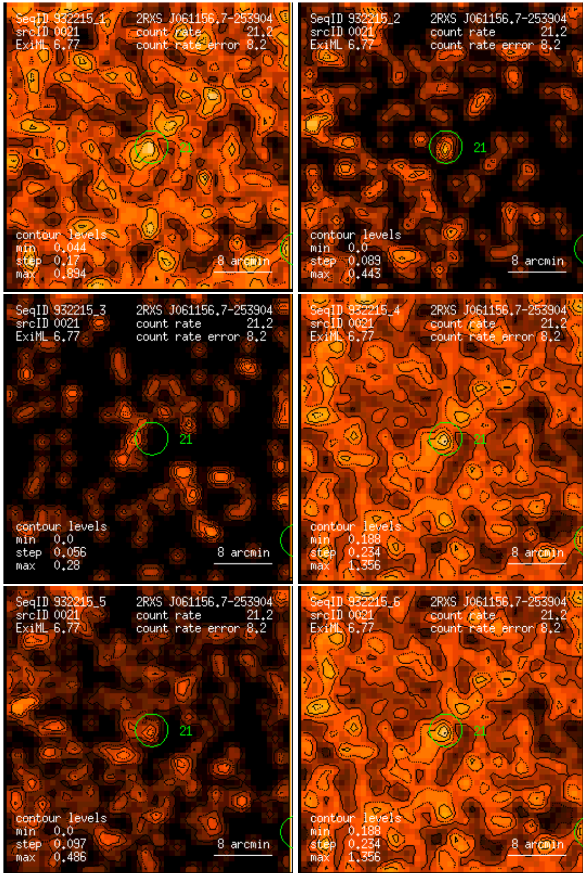
Figure 21: RASS 932215: detection 0021: band rate images, Gaussian filter: (1) PSPC channels 11 – 41, (2) 52 – 90, (3) 91 – 201, (4) 11 – 235, (5) 52 – 201, (6) 11 – 201. Broad band rates in counts/ks. Band rate contour levels in counts/ks/arcmin 2 .
