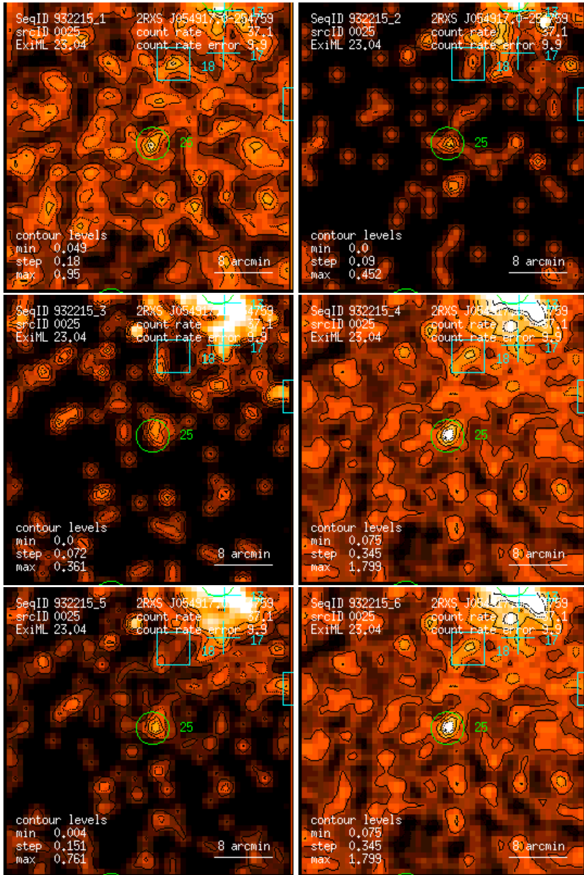
Figure 25: RASS 932215: detection 0025: band rate images, Gaussian filter: (1) PSPC channels 11 – 41, (2) 52 – 90, (3) 91 – 201, (4) 11 – 235, (5) 52 – 201, (6) 11 – 201. Broad band rates in counts/ks. Band rate contour levels in counts/ks/arcmin 2 .
