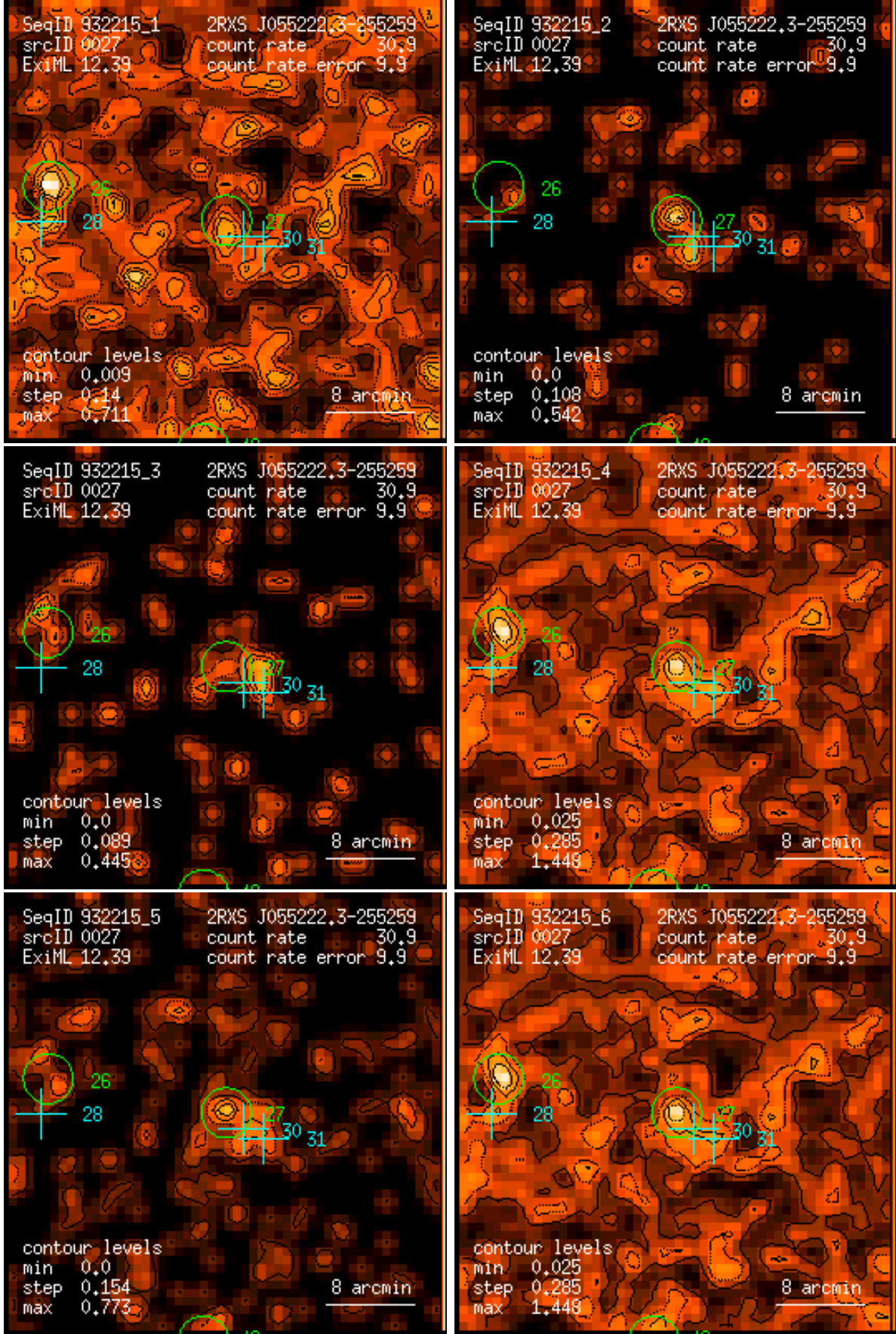
Figure 27: RASS 932215: detection 0027: band rate images, Gaussian filter: (1) PSPC channels 11 – 41, (2) 52 – 90, (3) 91 – 201, (4) 11 – 235, (5) 52 – 201, (6) 11 – 201. Broad band rates in counts/ks. Band rate contour levels in counts/ks/arcmin 2 .
