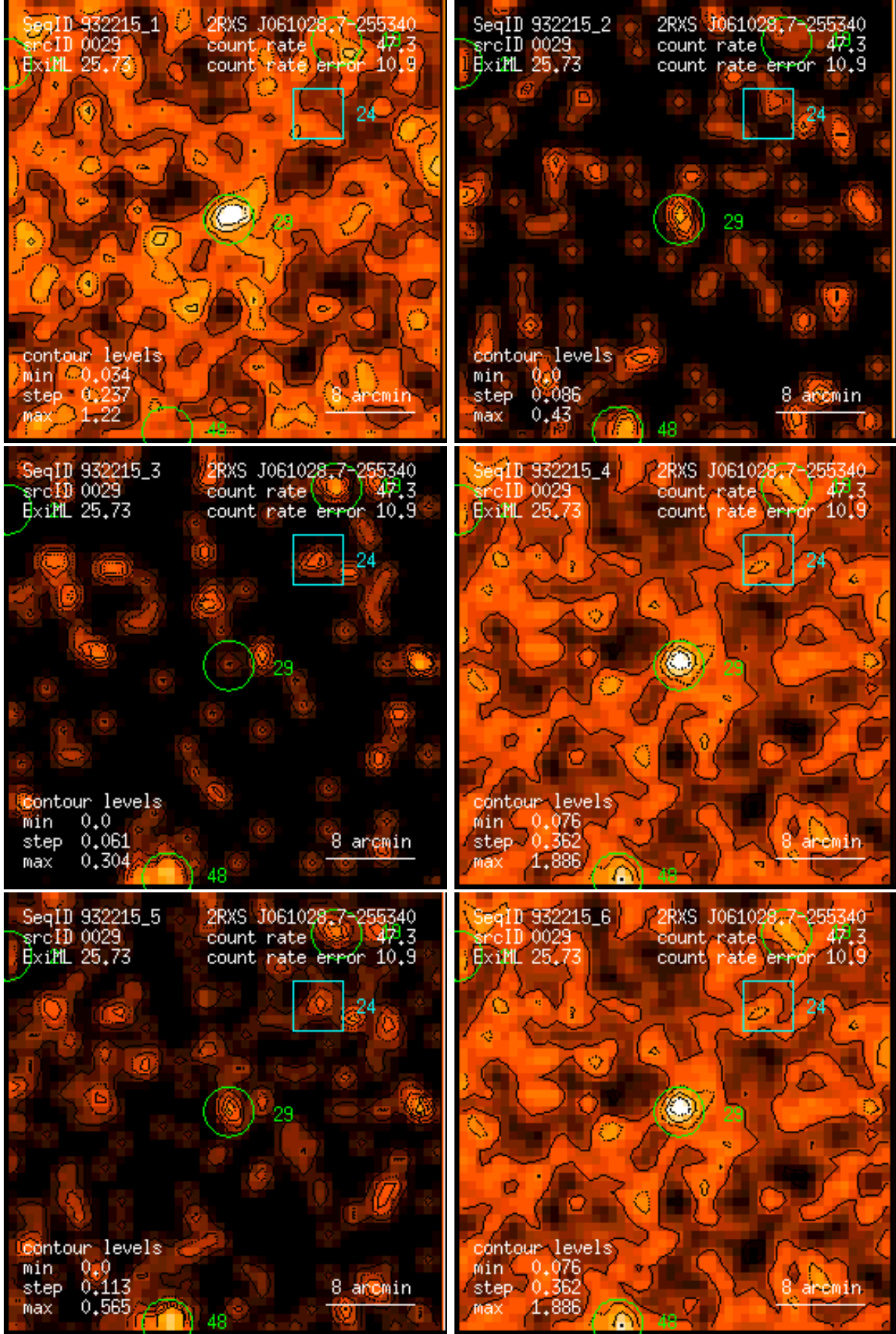
Figure 29: RASS 932215: detection 0029: band rate images, Gaussian filter: (1) PSPC channels 11 – 41, (2) 52 – 90, (3) 91 – 201, (4) 11 – 235, (5) 52 – 201, (6) 11 – 201. Broad band rates in counts/ks. Band rate contour levels in counts/ks/arcmin 2 .
