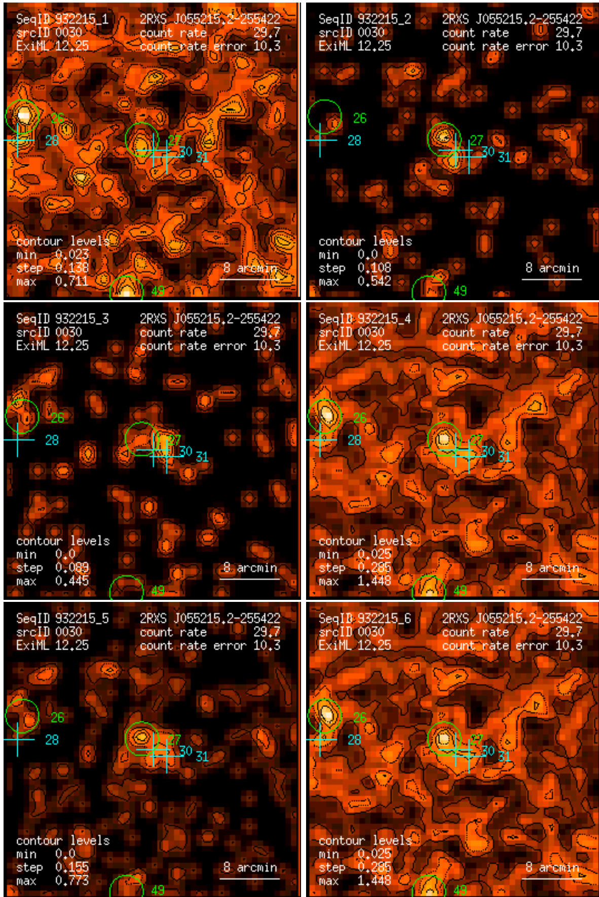
Figure 30: RASS 932215: detection 0030: band rate images, Gaussian filter: (1) PSPC channels 11 – 41, (2) 52 – 90, (3) 91 – 201, (4) 11 – 235, (5) 52 – 201, (6) 11 – 201. Broad band rates in counts/ks. Band rate contour levels in counts/ks/arcmin 2 .
