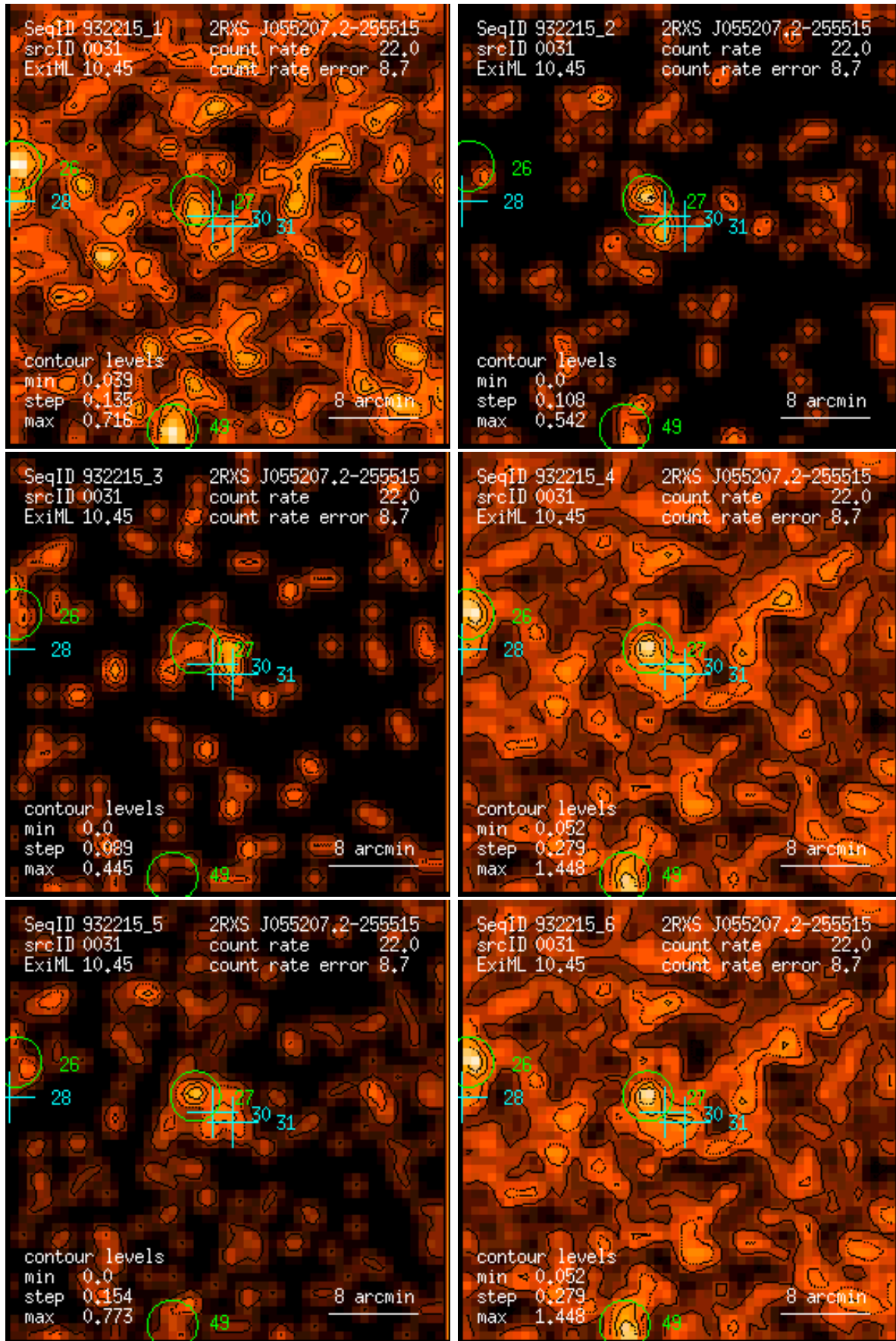
Figure 31: RASS 932215: detection 0031: band rate images, Gaussian filter: (1) PSPC channels 11 – 41, (2) 52 – 90, (3) 91 – 201, (4) 11 – 235, (5) 52 – 201, (6) 11 – 201. Broad band rates in counts/ks. Band rate contour levels in counts/ks/arcmin 2 .
