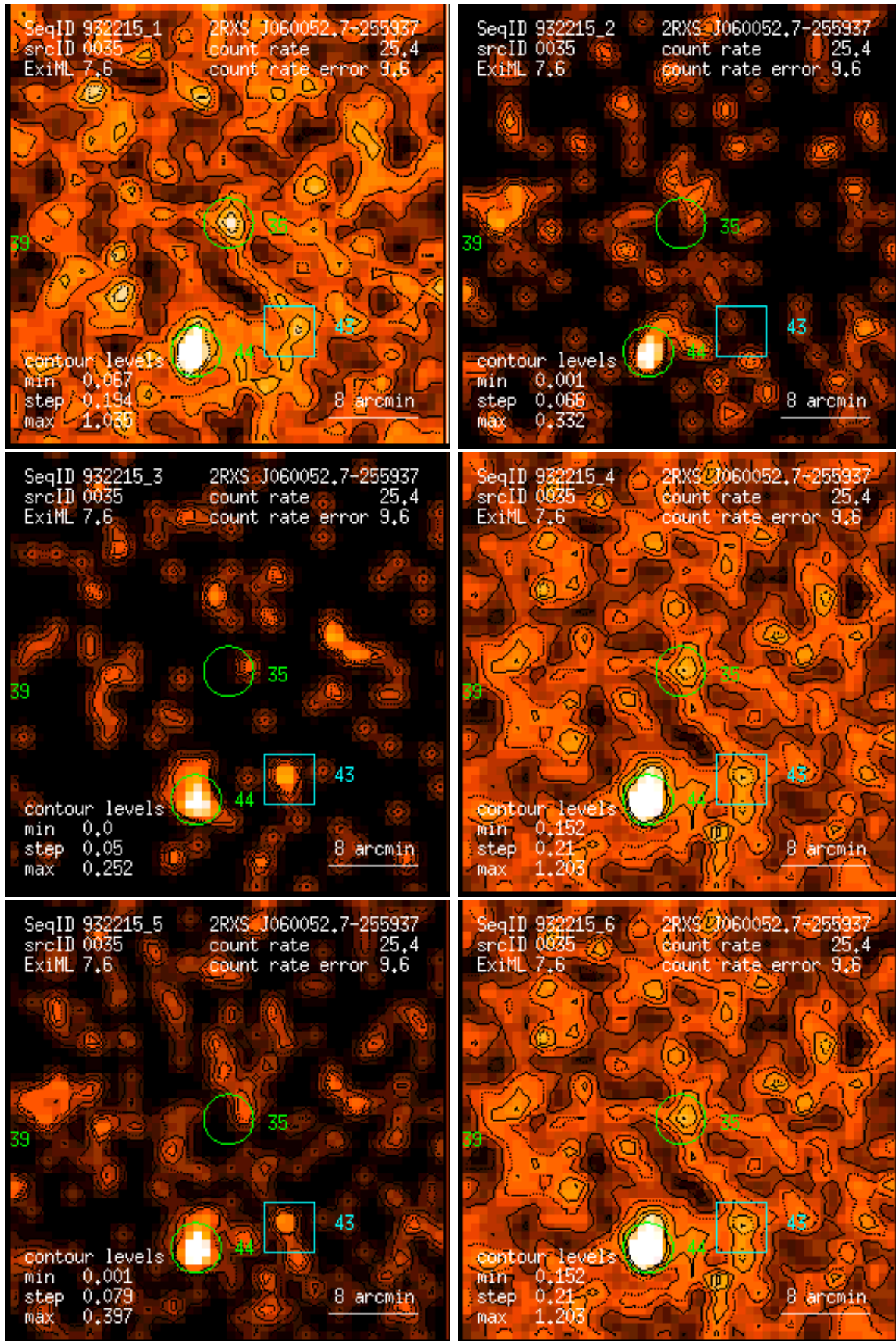
Figure 35: RASS 932215: detection 0035: band rate images, Gaussian filter: (1) PSPC channels 11 – 41, (2) 52 – 90, (3) 91 – 201, (4) 11 – 235, (5) 52 – 201, (6) 11 – 201. Broad band rates in counts/ks. Band rate contour levels in counts/ks/arcmin 2 .
