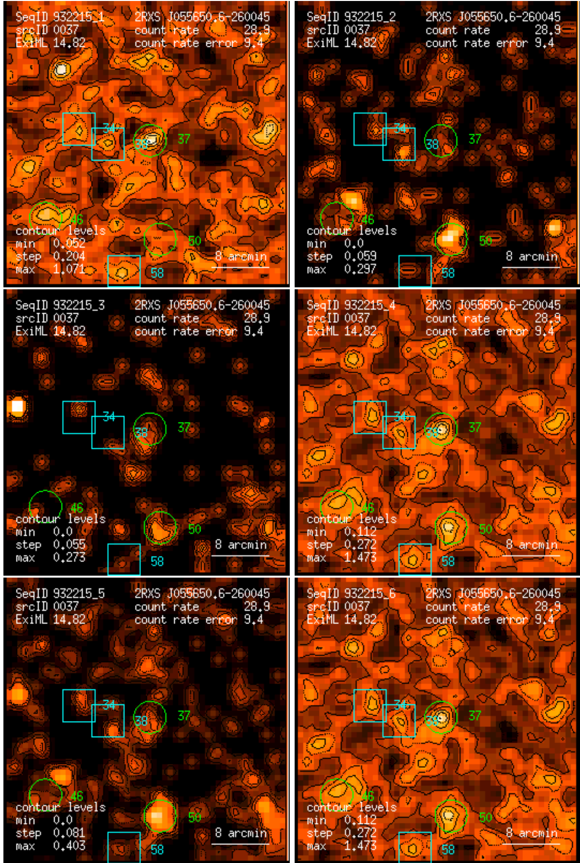
Figure 37: RASS 932215: detection 0037: band rate images, Gaussian filter: (1) PSPC channels 11 – 41, (2) 52 – 90, (3) 91 – 201, (4) 11 – 235, (5) 52 – 201, (6) 11 – 201. Broad band rates in counts/ks. Band rate contour levels in counts/ks/arcmin 2 .
