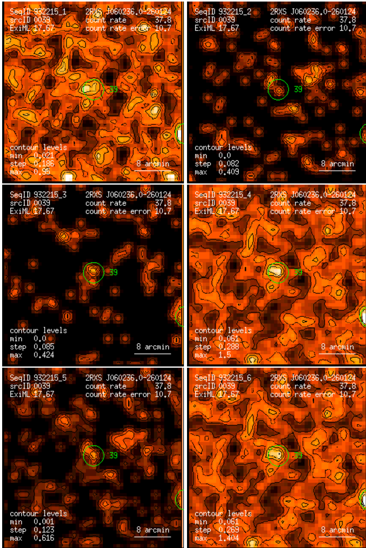
Figure 39: RASS 932215: detection 0039: band rate images, Gaussian filter: (1) PSPC channels 11 – 41, (2) 52 – 90, (3) 91 – 201, (4) 11 – 235, (5) 52 – 201, (6) 11 – 201. Broad band rates in counts/ks. Band rate contour levels in counts/ks/arcmin 2 .
