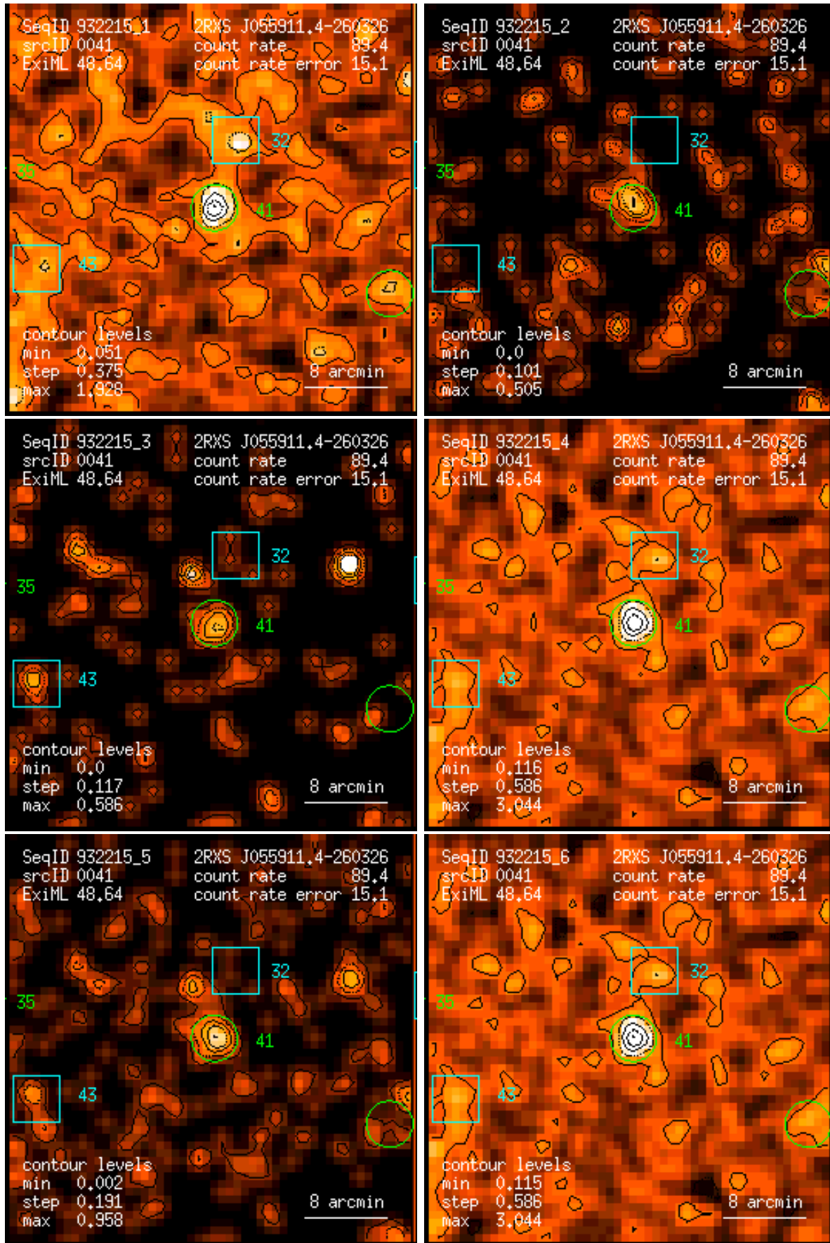
Figure 41: RASS 932215: detection 0041: band rate images, Gaussian filter: (1) PSPC channels 11 – 41, (2) 52 – 90, (3) 91 – 201, (4) 11 – 235, (5) 52 – 201, (6) 11 – 201. Broad band rates in counts/ks. Band rate contour levels in counts/ks/arcmin 2 .
