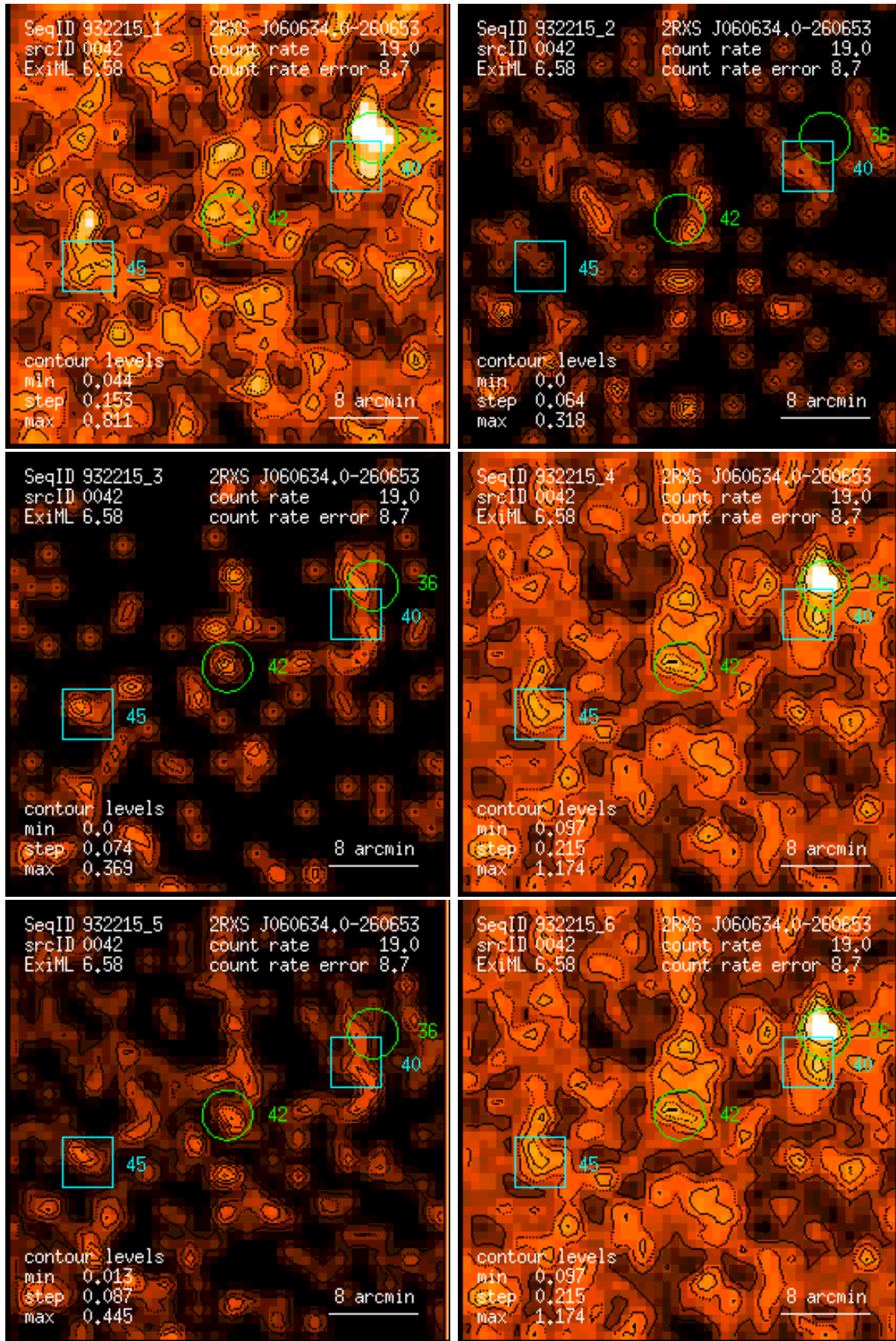
Figure 42: RASS 932215: detection 0042: band rate images, Gaussian filter: (1) PSPC channels 11 – 41, (2) 52 – 90, (3) 91 – 201, (4) 11 – 235, (5) 52 – 201, (6) 11 – 201. Broad band rates in counts/ks. Band rate contour levels in counts/ks/arcmin 2 .
