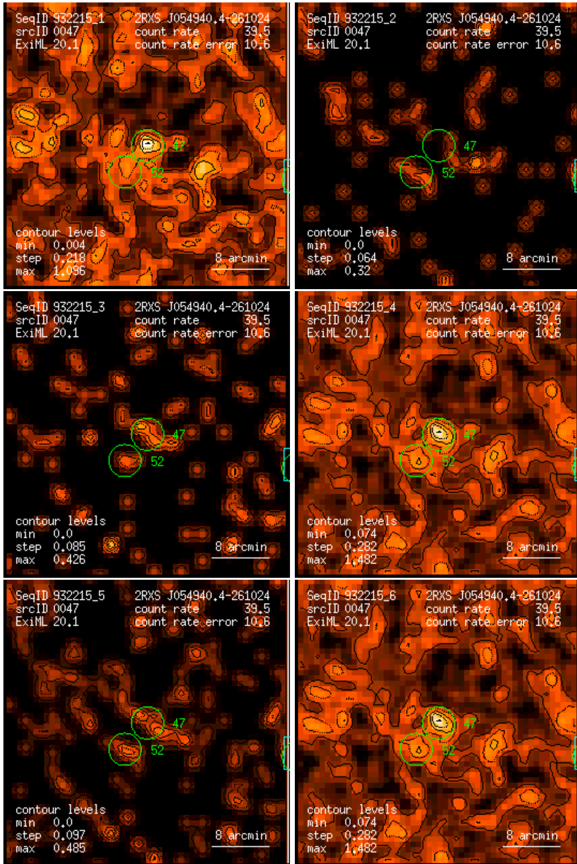
Figure 47: RASS 932215: detection 0047: band rate images, Gaussian filter: (1) PSPC channels 11 – 41, (2) 52 – 90, (3) 91 – 201, (4) 11 – 235, (5) 52 – 201, (6) 11 – 201. Broad band rates in counts/ks. Band rate contour levels in counts/ks/arcmin 2 .
