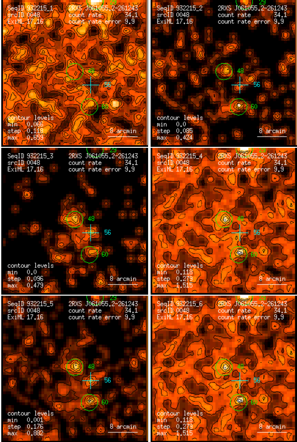
Figure 48: RASS 932215: detection 0048: band rate images, Gaussian filter: (1) PSPC channels 11 – 41, (2) 52 – 90, (3) 91 – 201, (4) 11 – 235, (5) 52 – 201, (6) 11 – 201. Broad band rates in counts/ks. Band rate contour levels in counts/ks/arcmin 2 .
