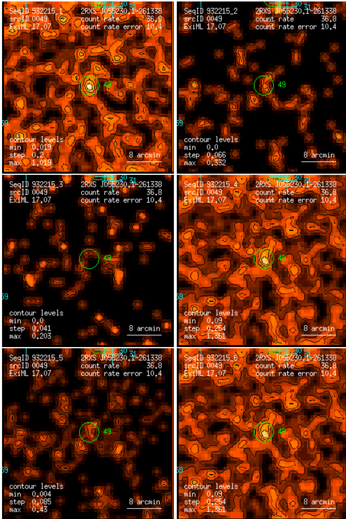
Figure 49: RASS 932215: detection 0049: band rate images, Gaussian filter: (1) PSPC channels 11 – 41, (2) 52 – 90, (3) 91 – 201, (4) 11 – 235, (5) 52 – 201, (6) 11 – 201. Broad band rates in counts/ks. Band rate contour levels in counts/ks/arcmin 2 .
