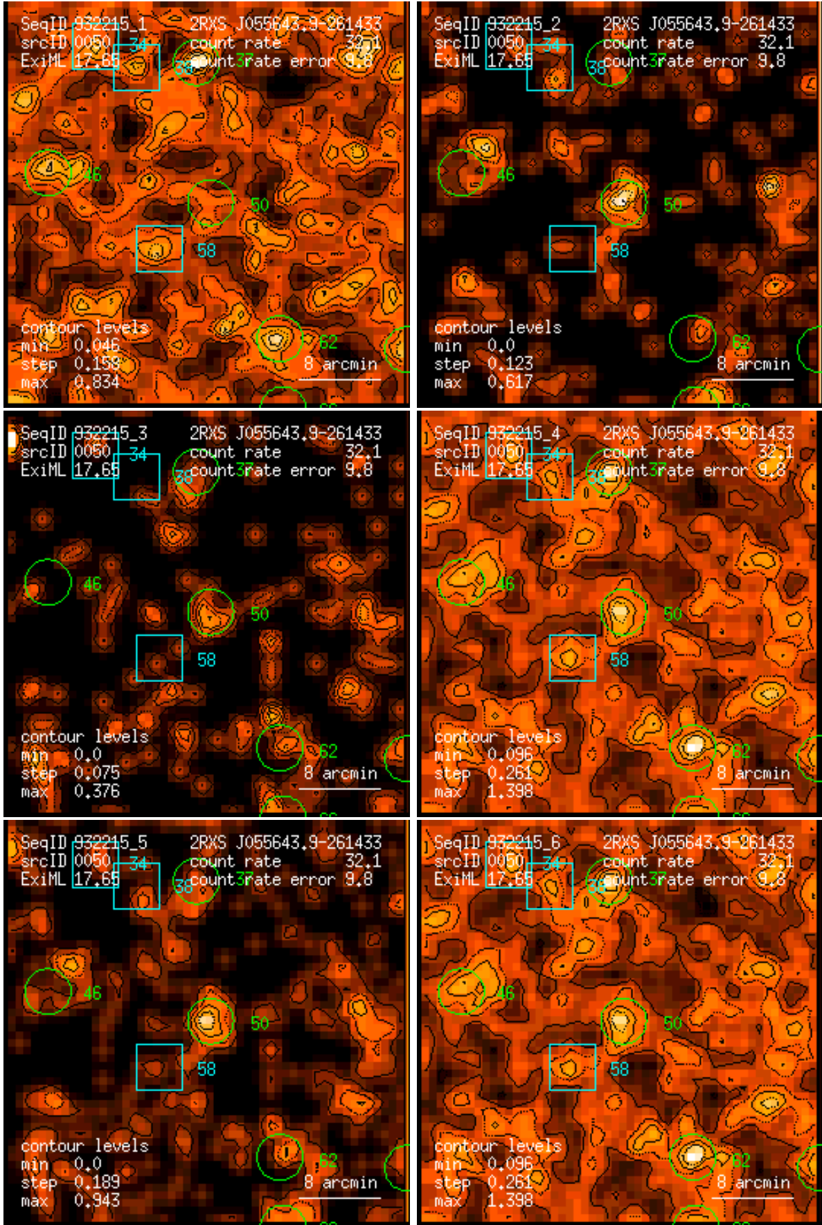
Figure 50: RASS 932215: detection 0050: band rate images, Gaussian filter: (1) PSPC channels 11 – 41, (2) 52 – 90, (3) 91 – 201, (4) 11 – 235, (5) 52 – 201, (6) 11 – 201. Broad band rates in counts/ks. Band rate contour levels in counts/ks/arcmin 2 .
