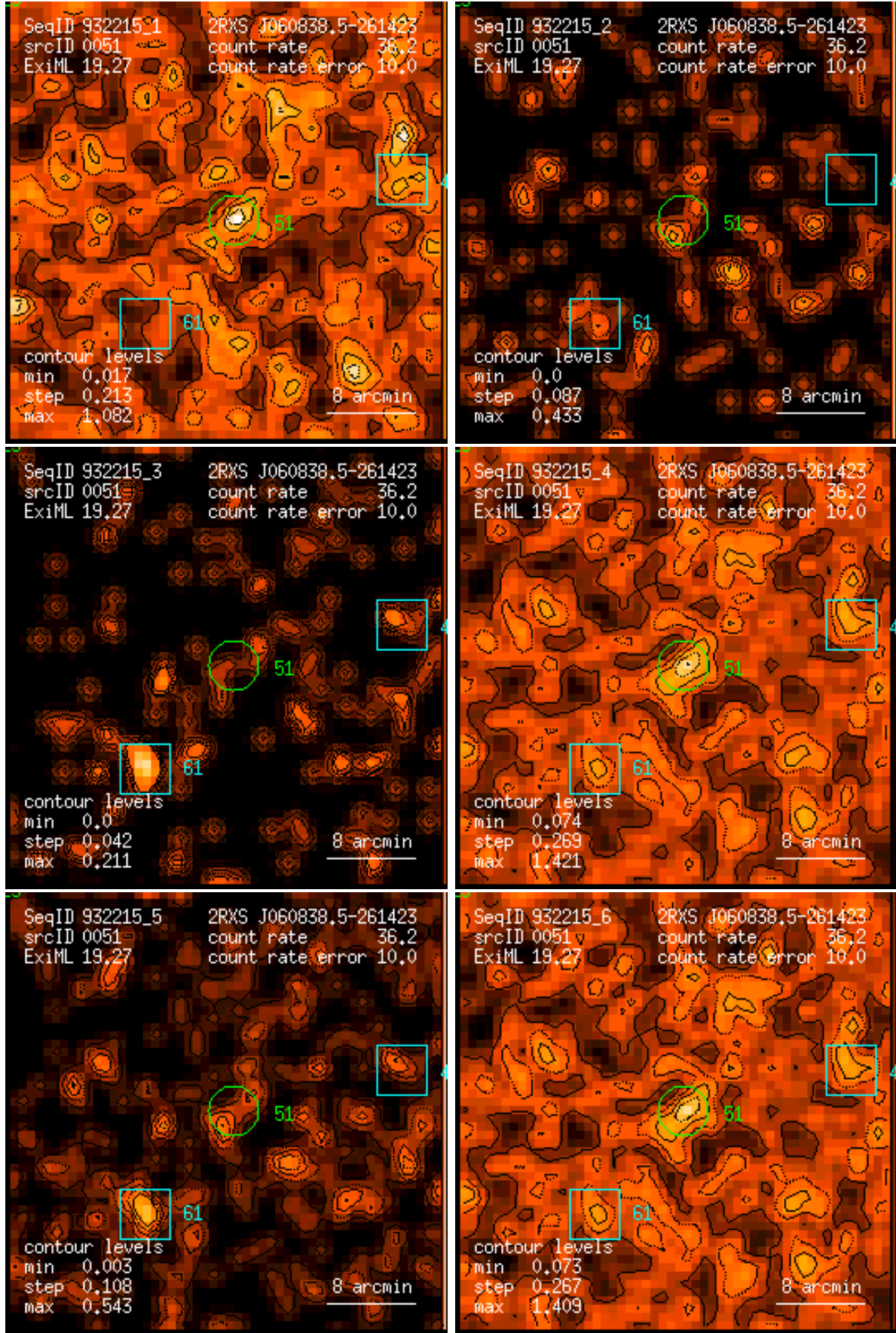
Figure 51: RASS 932215: detection 0051: band rate images, Gaussian filter: (1) PSPC channels 11 – 41, (2) 52 – 90, (3) 91 – 201, (4) 11 – 235, (5) 52 – 201, (6) 11 – 201. Broad band rates in counts/ks. Band rate contour levels in counts/ks/arcmin 2 .
