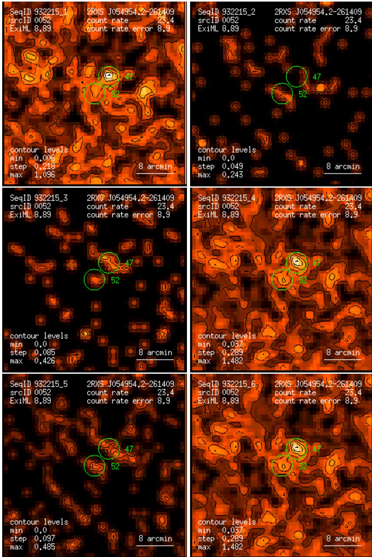
Figure 52: RASS 932215: detection 0052: band rate images, Gaussian filter: (1) PSPC channels 11 – 41, (2) 52 – 90, (3) 91 – 201, (4) 11 – 235, (5) 52 – 201, (6) 11 – 201. Broad band rates in counts/ks. Band rate contour levels in counts/ks/arcmin 2 .
