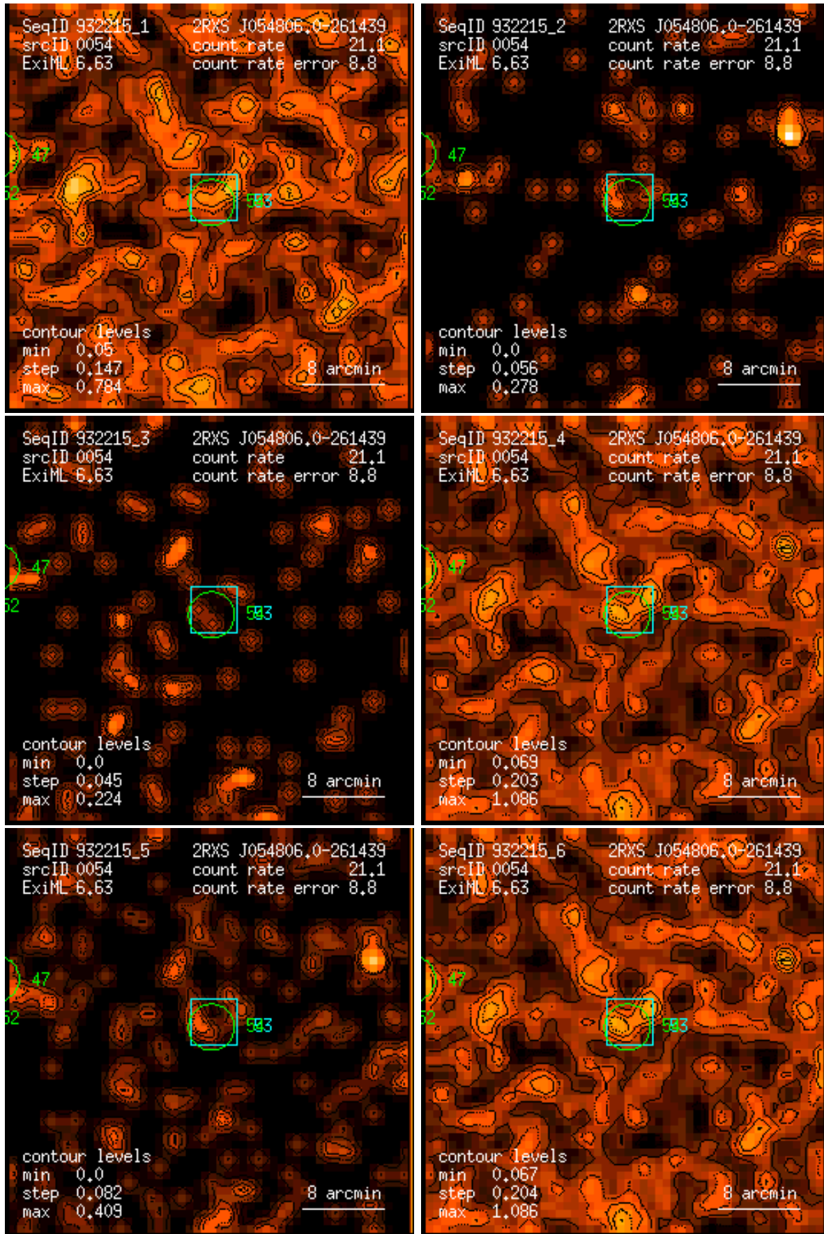
Figure 54: RASS 932215: detection 0054: band rate images, Gaussian filter: (1) PSPC channels 11 – 41, (2) 52 – 90, (3) 91 – 201, (4) 11 – 235, (5) 52 – 201, (6) 11 – 201. Broad band rates in counts/ks. Band rate contour levels in counts/ks/arcmin 2 .
