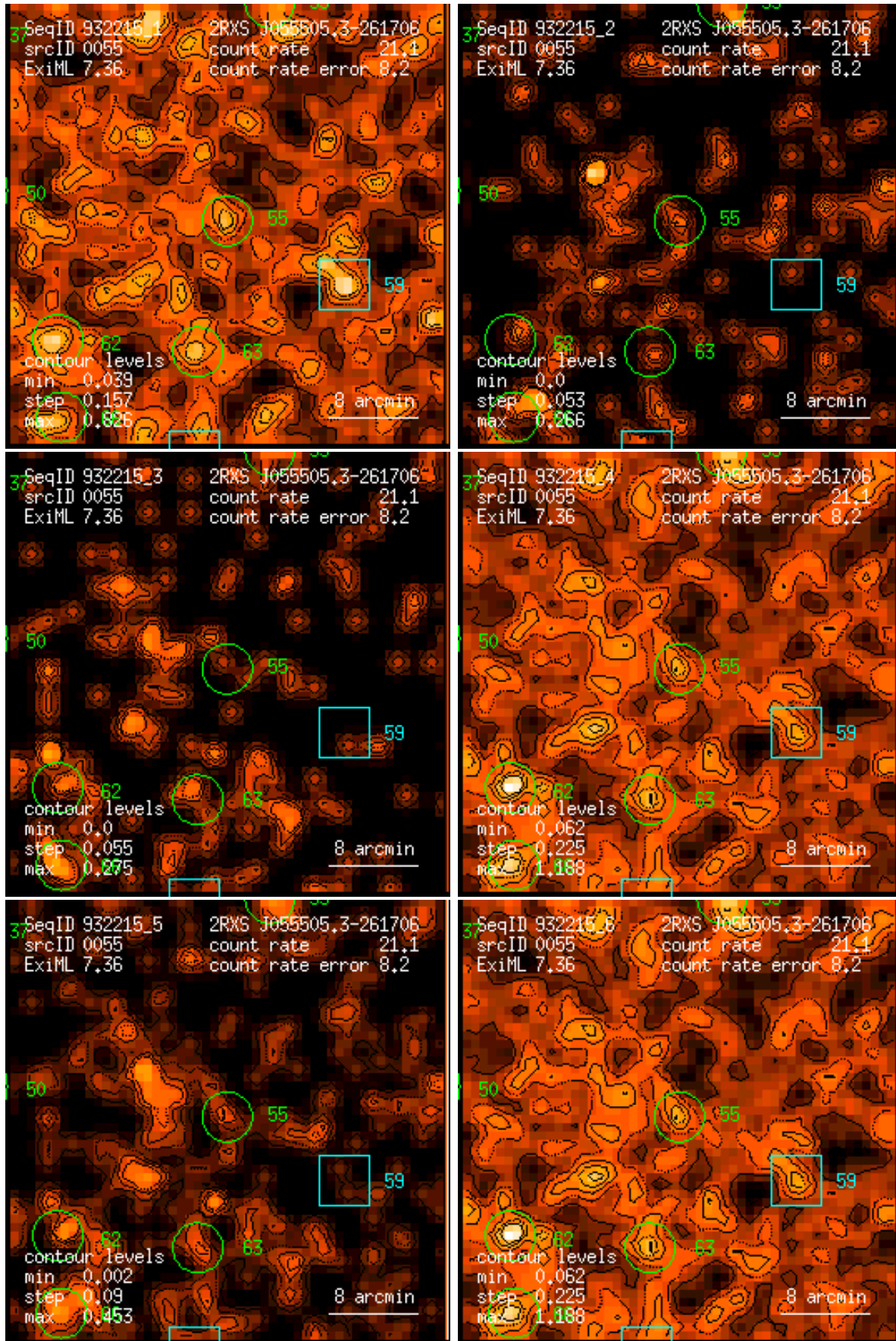
Figure 55: RASS 932215: detection 0055: band rate images, Gaussian filter: (1) PSPC channels 11 – 41, (2) 52 – 90, (3) 91 – 201, (4) 11 – 235, (5) 52 – 201, (6) 11 – 201. Broad band rates in counts/ks. Band rate contour levels in counts/ks/arcmin 2 .
