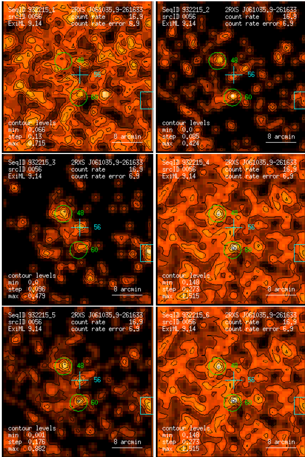
Figure 56: RASS 932215: detection 0056: band rate images, Gaussian filter: (1) PSPC channels 11 – 41, (2) 52 – 90, (3) 91 – 201, (4) 11 – 235, (5) 52 – 201, (6) 11 – 201. Broad band rates in counts/ks. Band rate contour levels in counts/ks/arcmin 2 .
