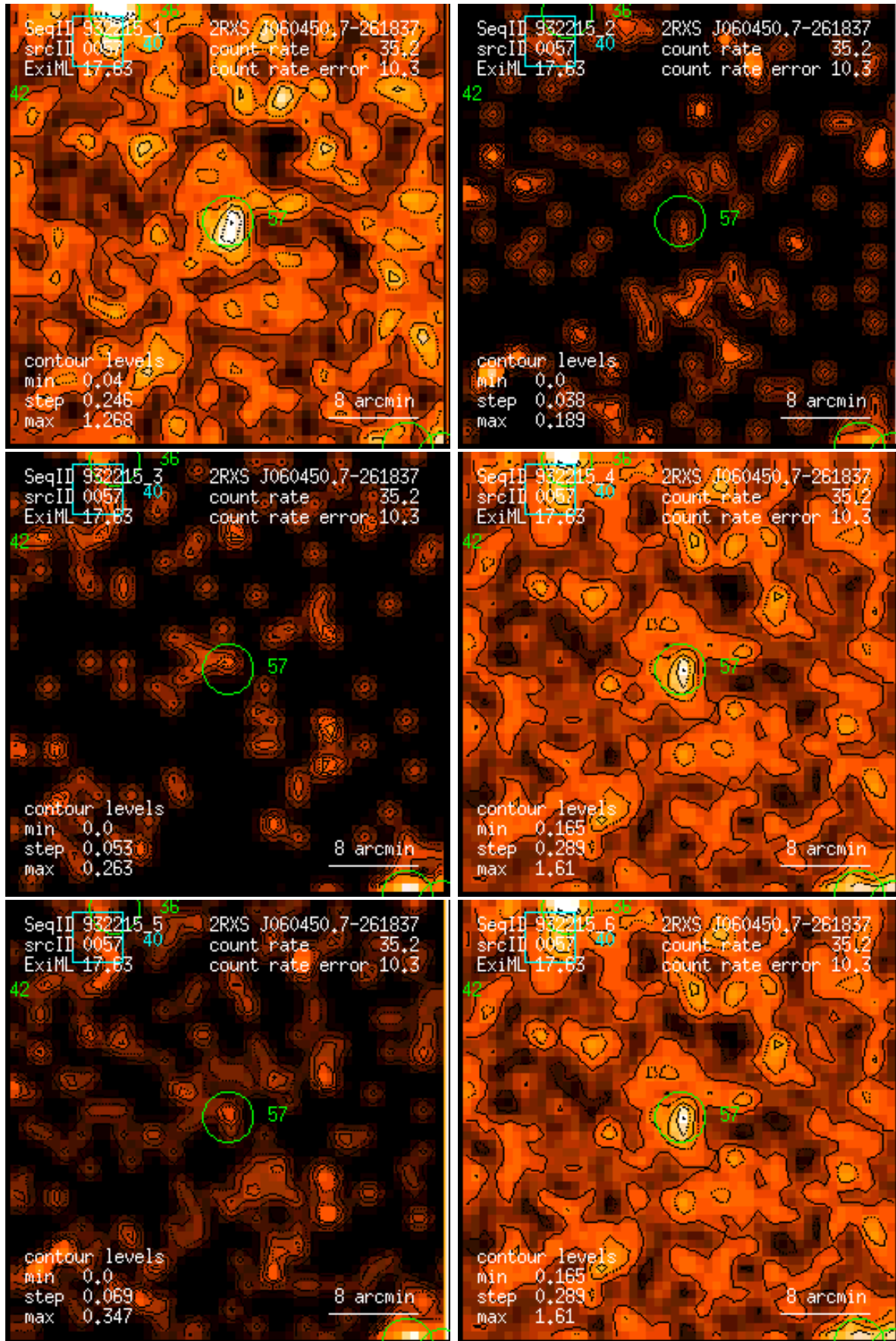
Figure 57: RASS 932215: detection 0057: band rate images, Gaussian filter: (1) PSPC channels 11 – 41, (2) 52 – 90, (3) 91 – 201, (4) 11 – 235, (5) 52 – 201, (6) 11 – 201. Broad band rates in counts/ks. Band rate contour levels in counts/ks/arcmin 2 .
