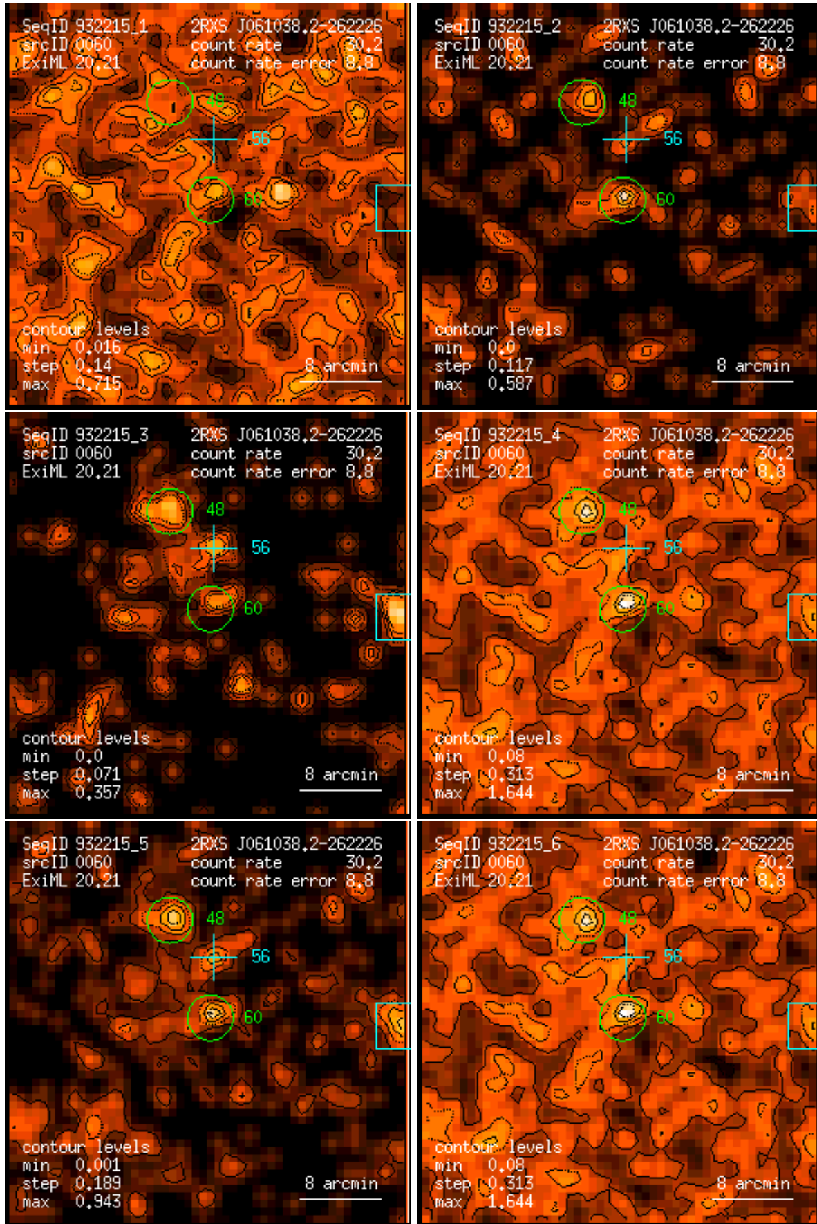
Figure 60: RASS 932215: detection 0060: band rate images, Gaussian filter: (1) PSPC channels 11 – 41, (2) 52 – 90, (3) 91 – 201, (4) 11 – 235, (5) 52 – 201, (6) 11 – 201. Broad band rates in counts/ks. Band rate contour levels in counts/ks/arcmin 2 .
