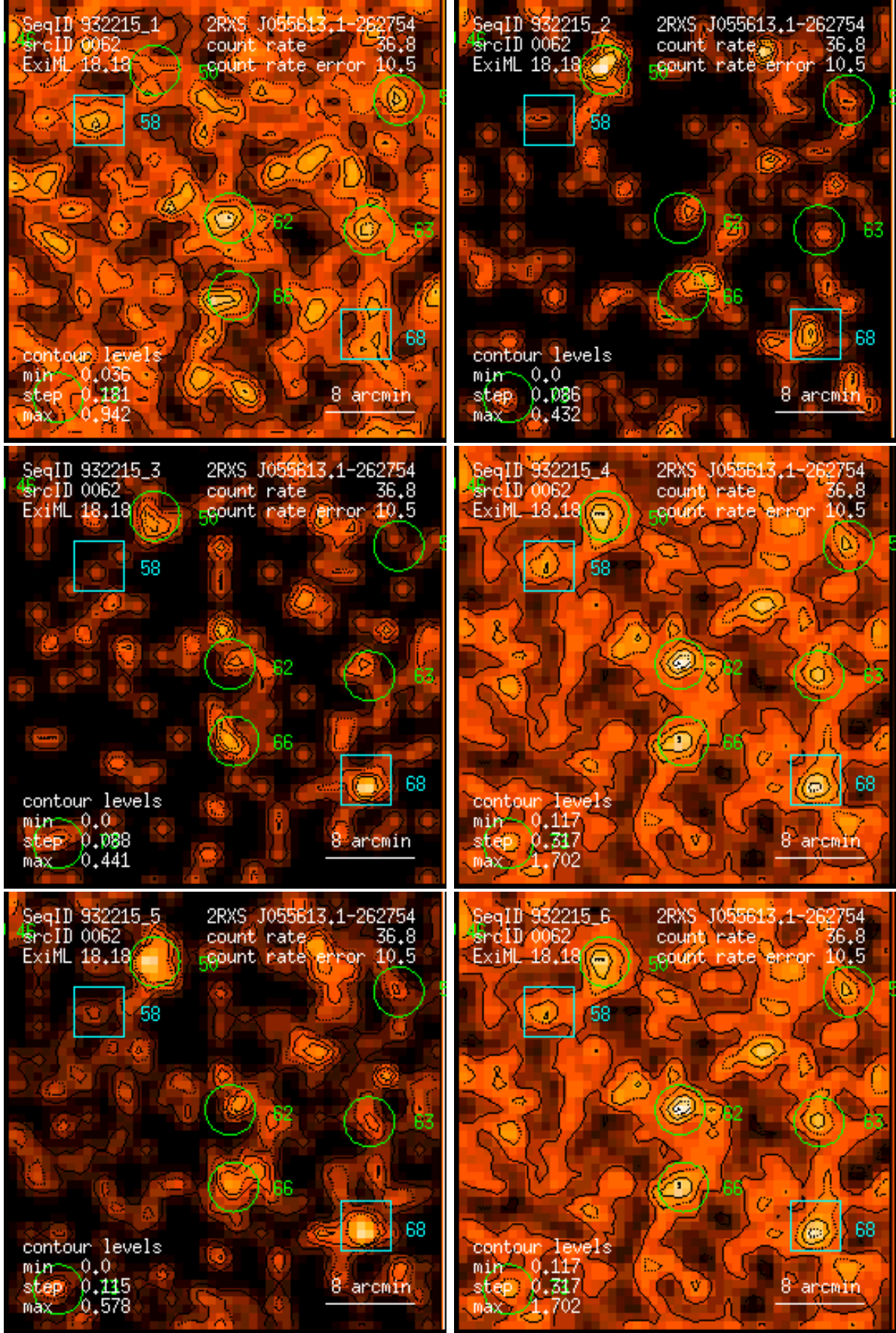
Figure 62: RASS 932215: detection 0062: band rate images, Gaussian filter: (1) PSPC channels 11 – 41, (2) 52 – 90, (3) 91 – 201, (4) 11 – 235, (5) 52 – 201, (6) 11 – 201. Broad band rates in counts/ks. Band rate contour levels in counts/ks/arcmin 2 .
