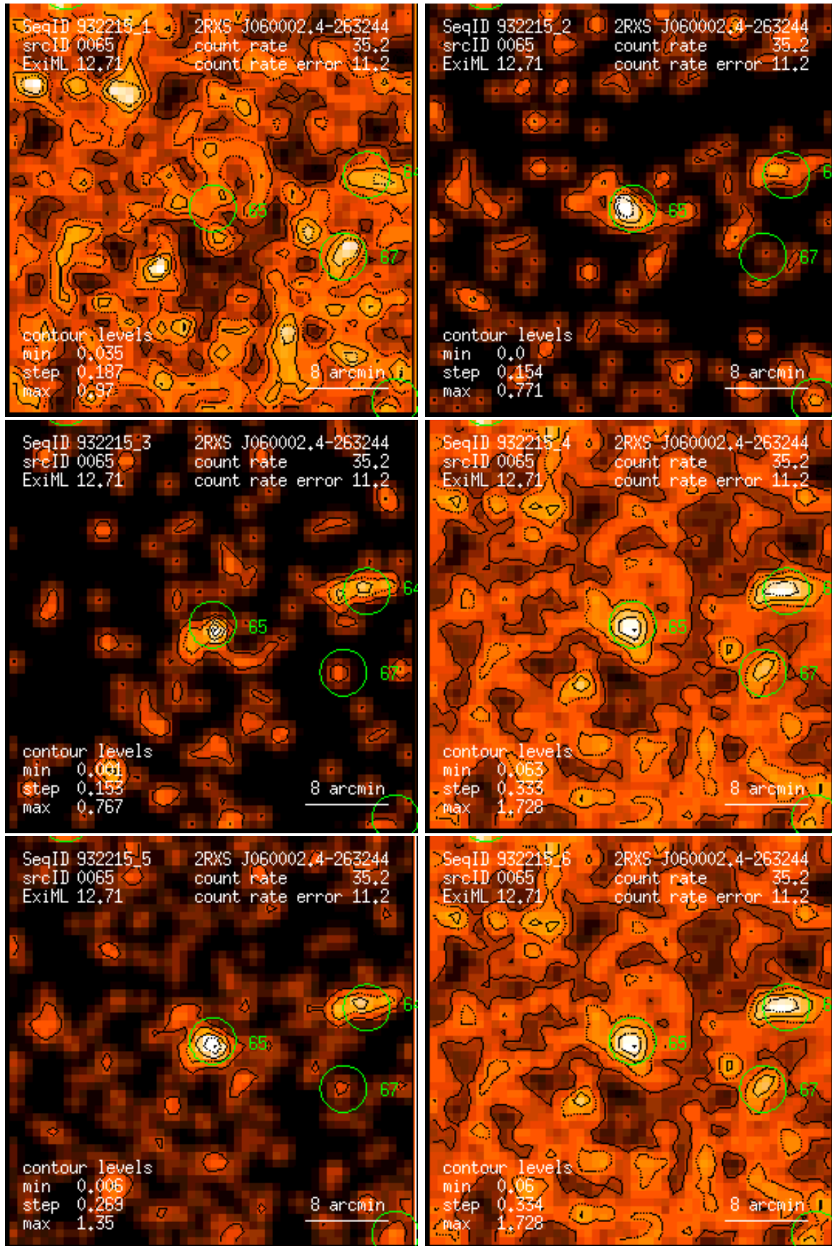
Figure 65: RASS 932215: detection 0065: band rate images, Gaussian filter: (1) PSPC channels 11 – 41, (2) 52 – 90, (3) 91 – 201, (4) 11 – 235, (5) 52 – 201, (6) 11 – 201. Broad band rates in counts/ks. Band rate contour levels in counts/ks/arcmin 2 .
