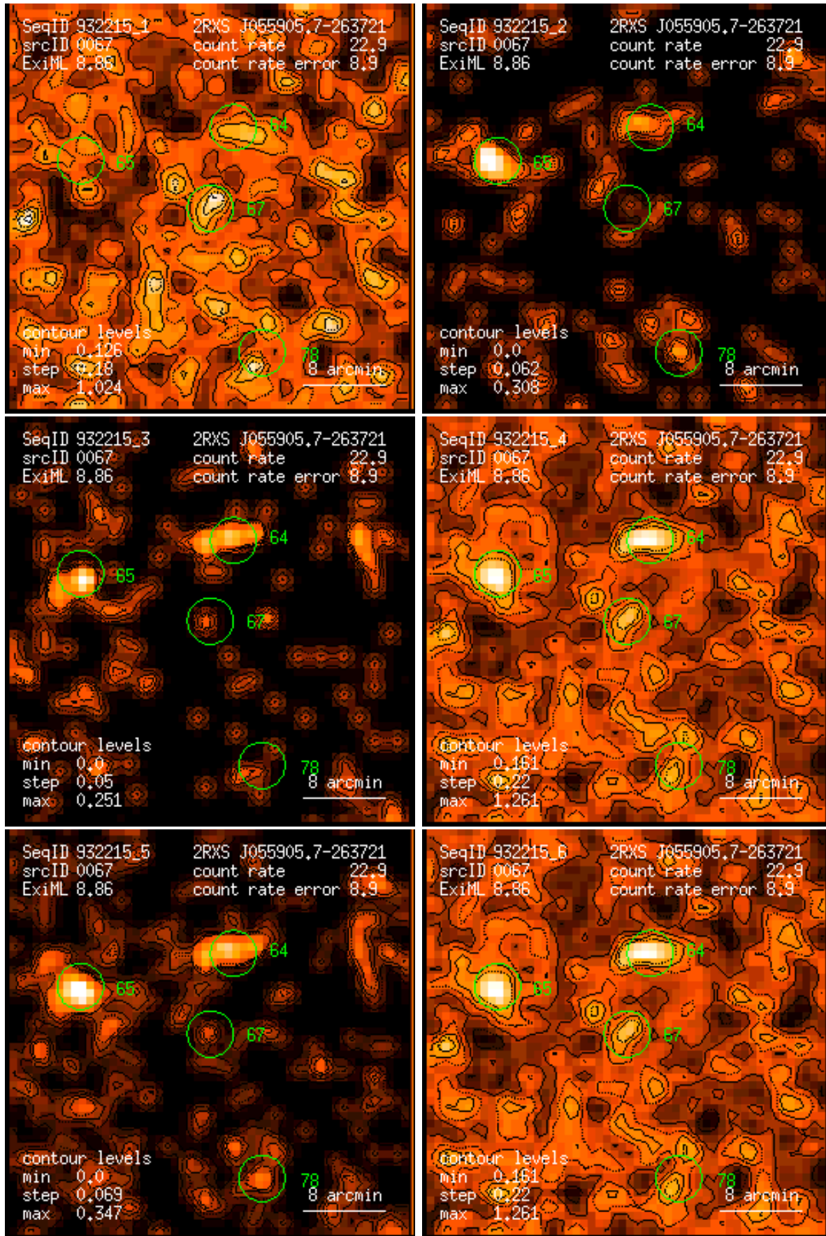
Figure 67: RASS 932215: detection 0067: band rate images, Gaussian filter: (1) PSPC channels 11 – 41, (2) 52 – 90, (3) 91 – 201, (4) 11 – 235, (5) 52 – 201, (6) 11 – 201. Broad band rates in counts/ks. Band rate contour levels in counts/ks/arcmin 2 .
