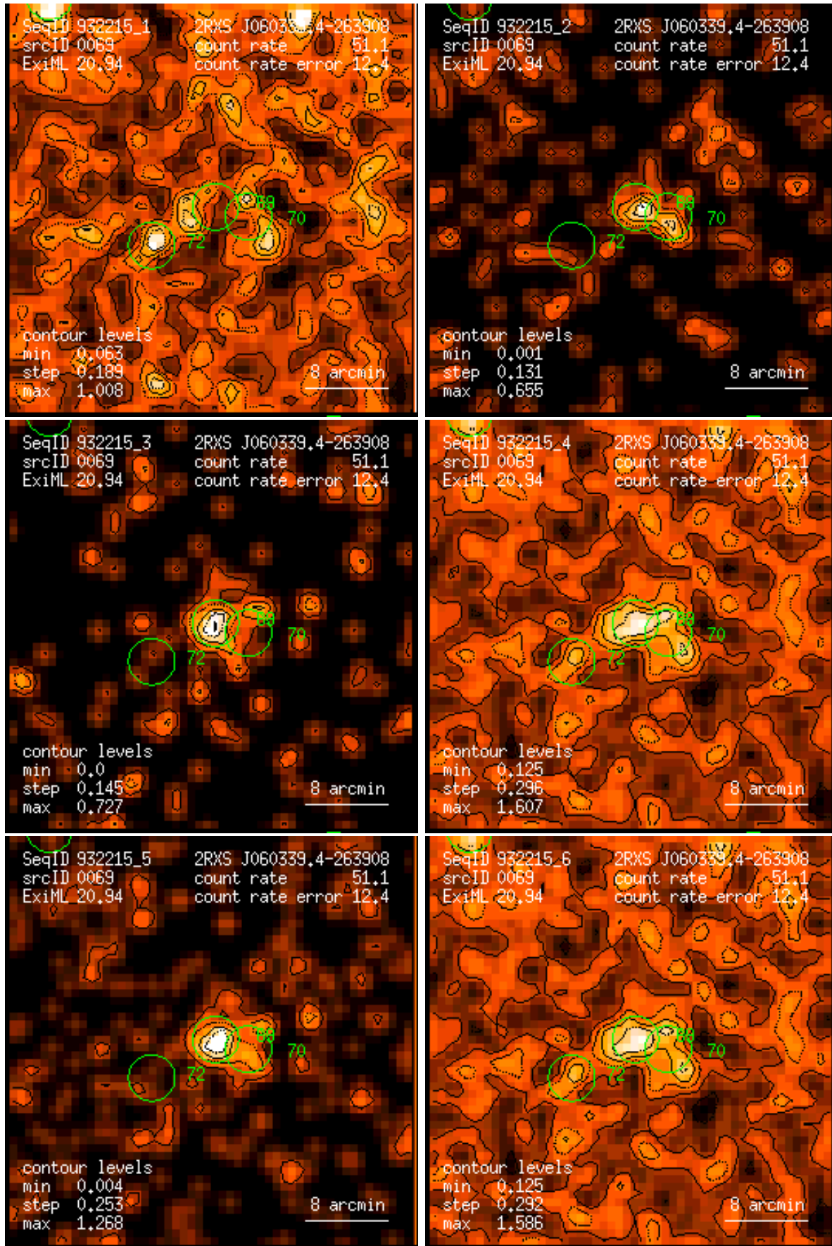
Figure 69: RASS 932215: detection 0069: band rate images, Gaussian filter: (1) PSPC channels 11 – 41, (2) 52 – 90, (3) 91 – 201, (4) 11 – 235, (5) 52 – 201, (6) 11 – 201. Broad band rates in counts/ks. Band rate contour levels in counts/ks/arcmin 2 .
