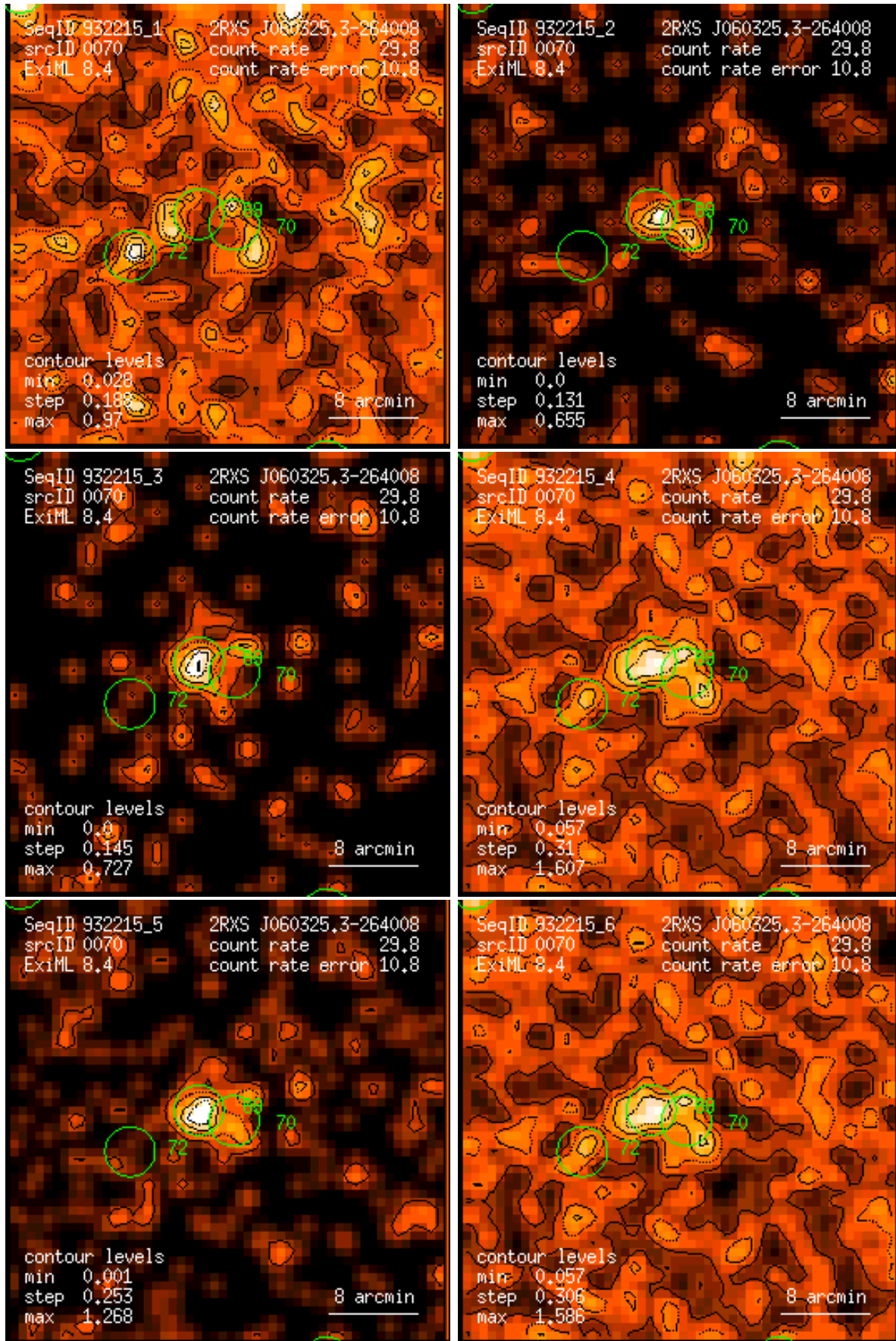
Figure 70: RASS 932215: detection 0070: band rate images, Gaussian filter: (1) PSPC channels 11 – 41, (2) 52 – 90, (3) 91 – 201, (4) 11 – 235, (5) 52 – 201, (6) 11 – 201. Broad band rates in counts/ks. Band rate contour levels in counts/ks/arcmin 2 .
