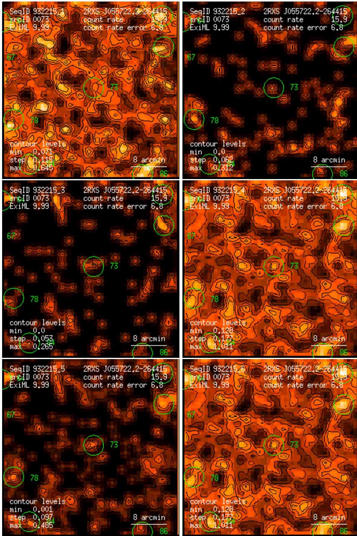
Figure 73: RASS 932215: detection 0073: band rate images, Gaussian filter: (1) PSPC channels 11 – 41, (2) 52 – 90, (3) 91 – 201, (4) 11 – 235, (5) 52 – 201, (6) 11 – 201. Broad band rates in counts/ks. Band rate contour levels in counts/ks/arcmin 2 .
