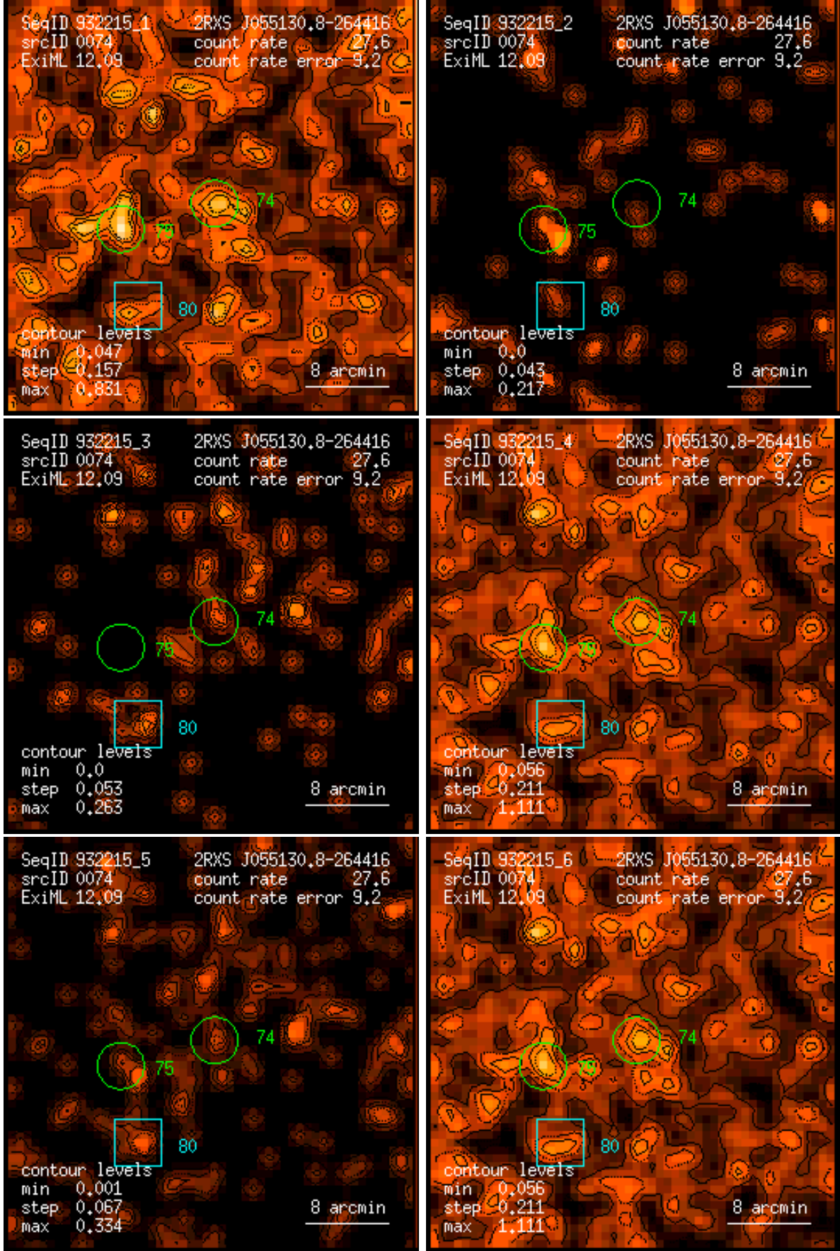
Figure 74: RASS 932215: detection 0074: band rate images, Gaussian filter: (1) PSPC channels 11 – 41, (2) 52 – 90, (3) 91 – 201, (4) 11 – 235, (5) 52 – 201, (6) 11 – 201. Broad band rates in counts/ks. Band rate contour levels in counts/ks/arcmin 2 .
