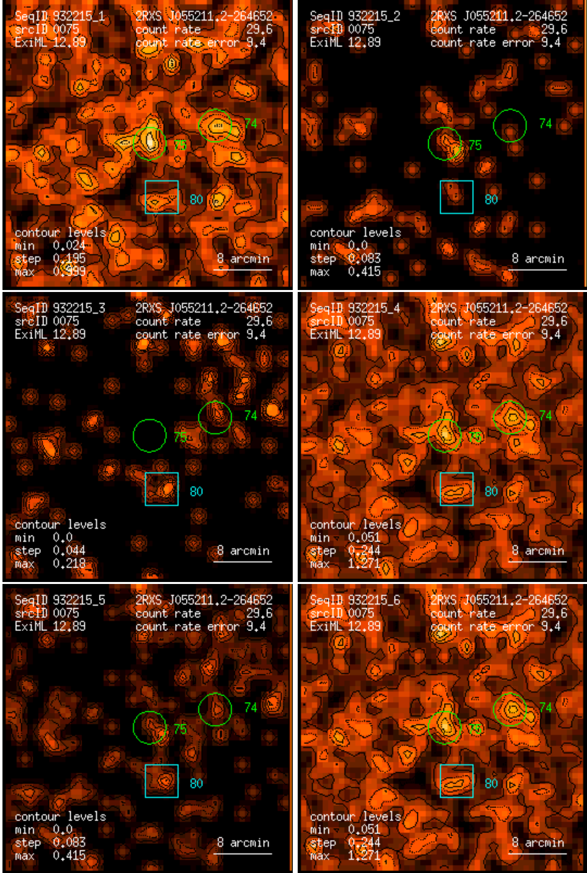
Figure 75: RASS 932215: detection 0075: band rate images, Gaussian filter: (1) PSPC channels 11 – 41, (2) 52 – 90, (3) 91 – 201, (4) 11 – 235, (5) 52 – 201, (6) 11 – 201. Broad band rates in counts/ks. Band rate contour levels in counts/ks/arcmin 2 .
