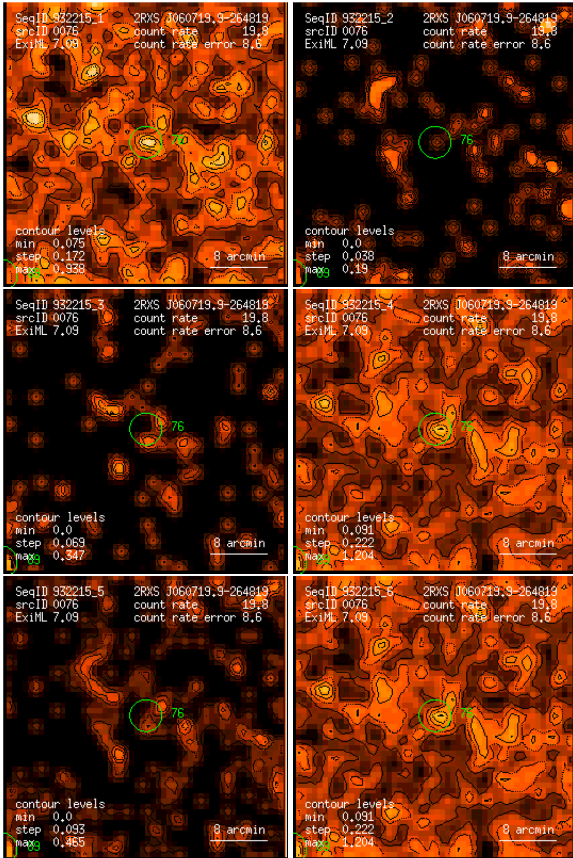
Figure 76: RASS 932215: detection 0076: band rate images, Gaussian filter: (1) PSPC channels 11 – 41, (2) 52 – 90, (3) 91 – 201, (4) 11 – 235, (5) 52 – 201, (6) 11 – 201. Broad band rates in counts/ks. Band rate contour levels in counts/ks/arcmin 2 .
